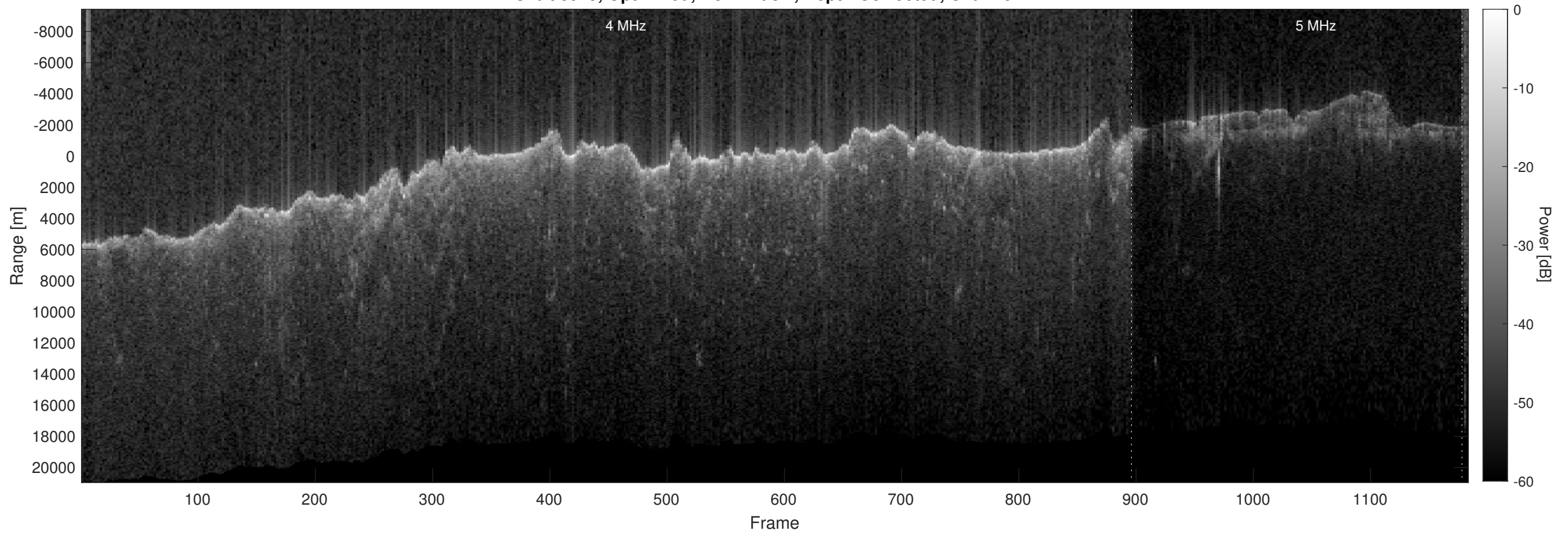
Orbit 8979, Optimized, No Window, Depth-Corrected, Channel 2
