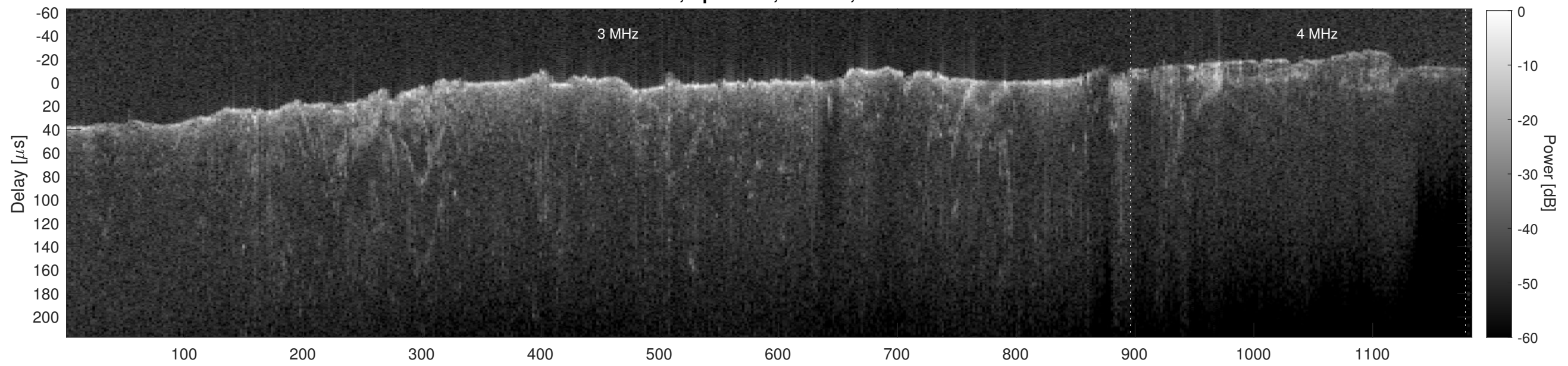
Orbit 8979, Cluttergram
