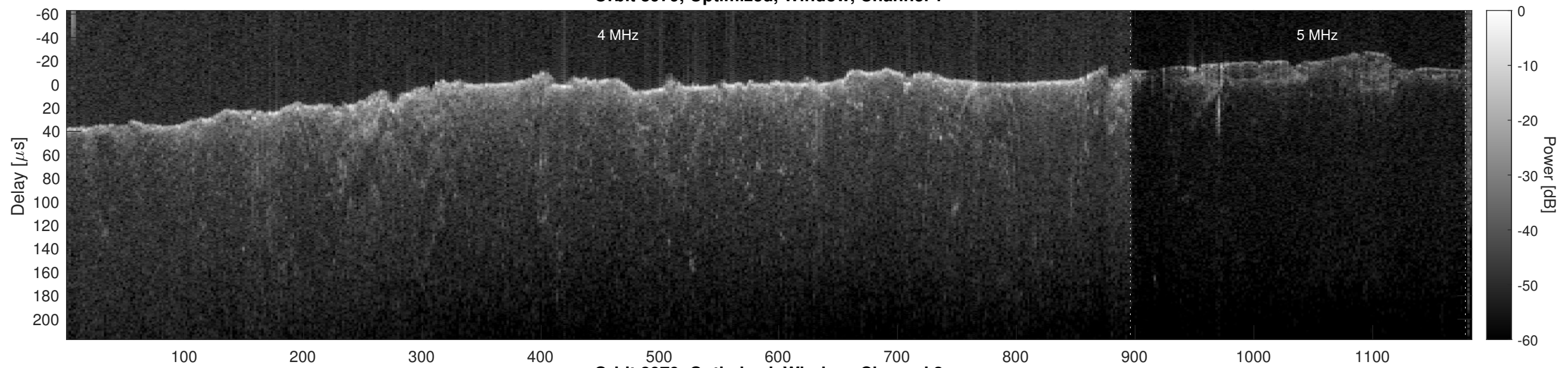
Orbit 8979, Optimized, Window, Channel 2
