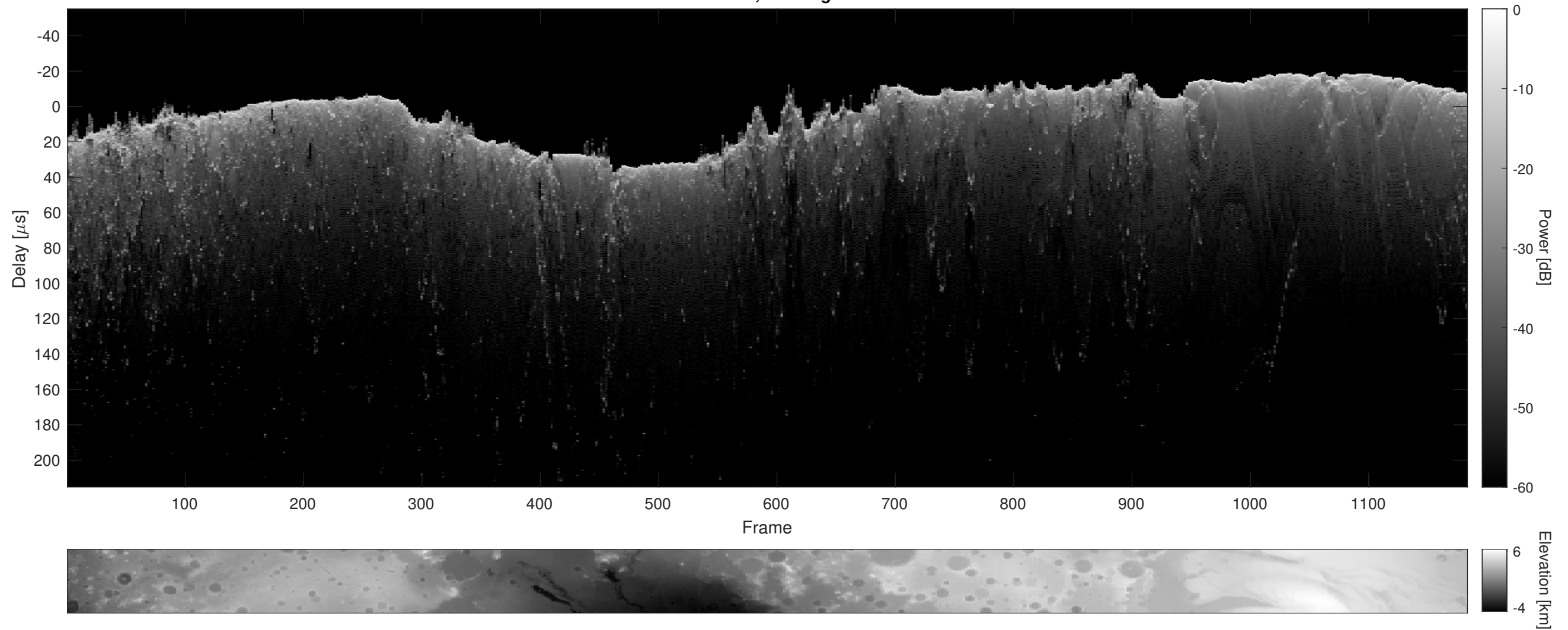
Orbit 8980, Cluttergram
