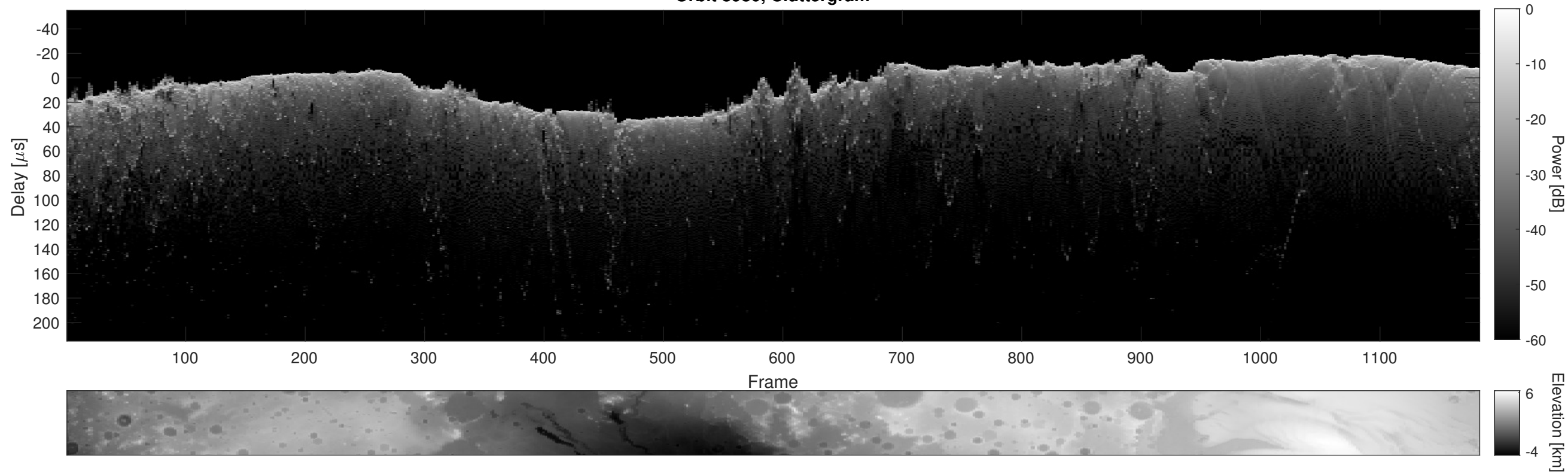
Orbit 8980, Cluttergram
