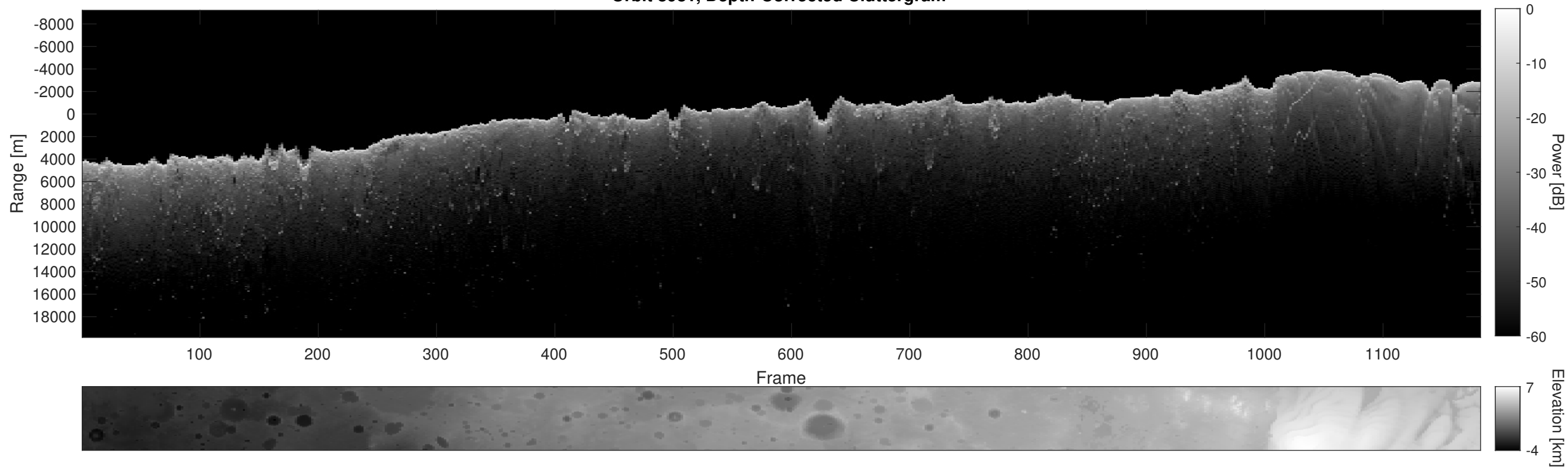
Orbit 8981, Depth-Corrected Cluttergram
