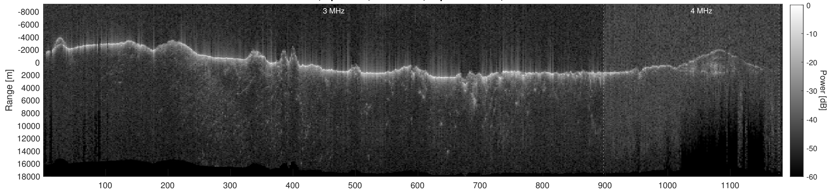
Orbit 8982, Depth-Corrected Cluttergram
