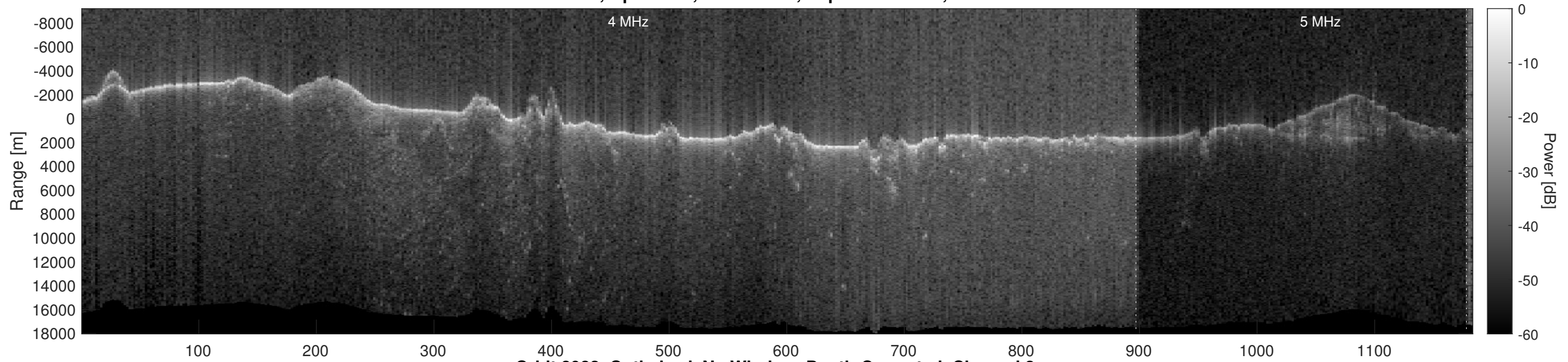
Orbit 8982, Optimized, No Window, Depth-Corrected, Channel 2
