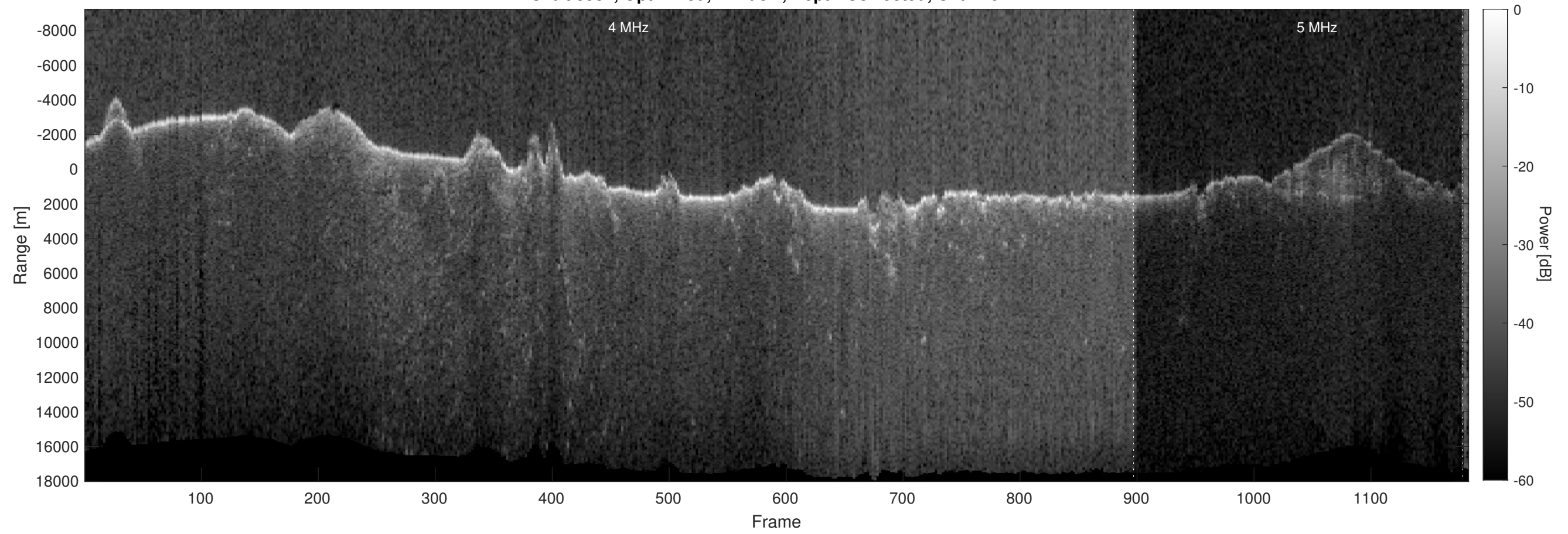
Orbit 8982, Optimized, Window, Depth-Corrected, Channel 2
