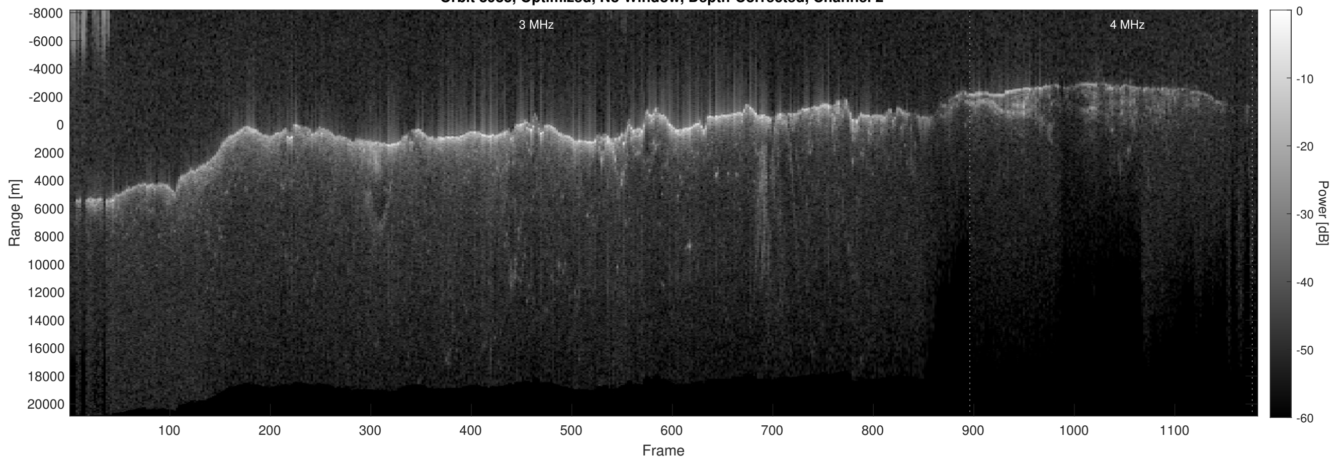
Orbit 8983, Optimized, No Window, Depth-Corrected, Channel 2
