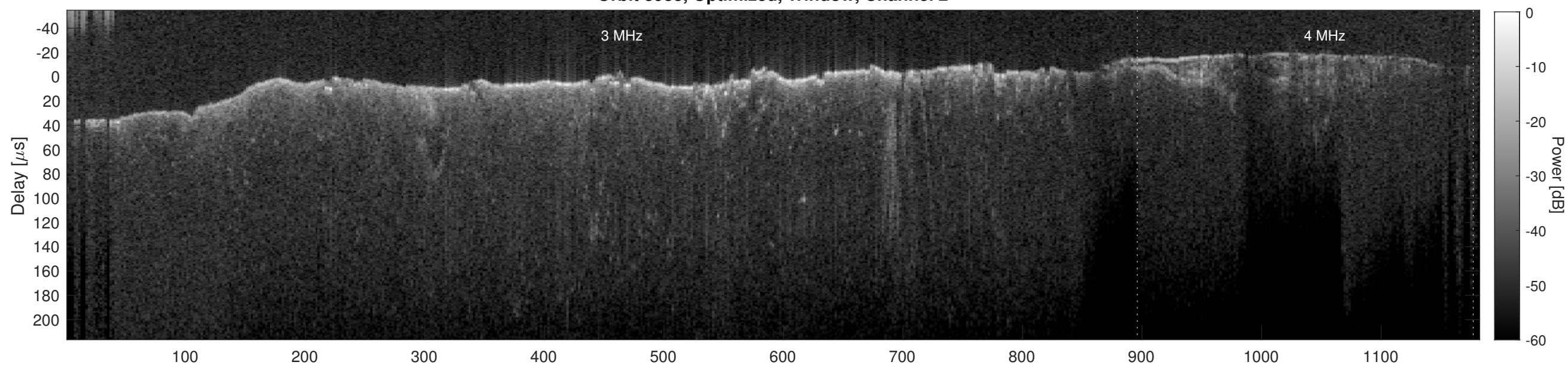
Orbit 8983, Cluttergram
