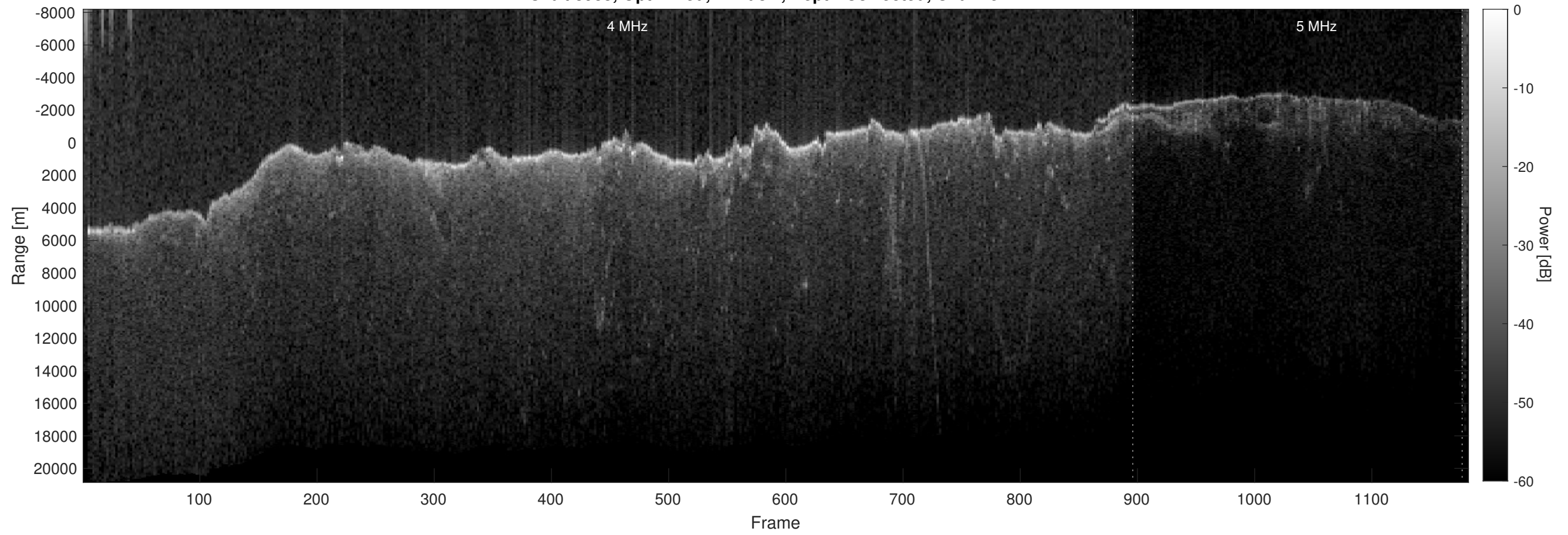
Orbit 8983, Optimized, Window, Depth-Corrected, Channel 2
