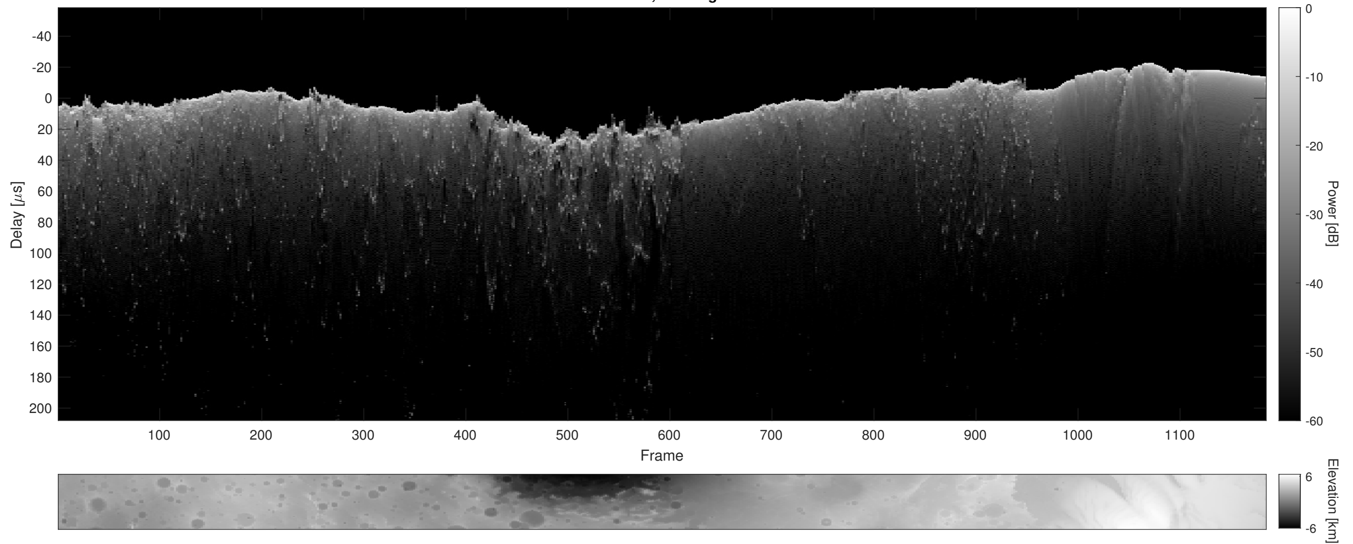
Orbit 8984, Cluttergram
