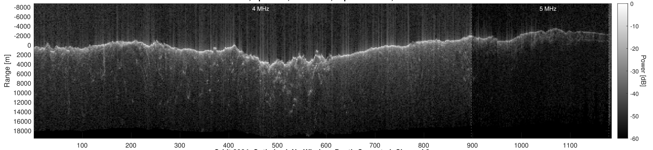
Orbit 8984, Optimized, No Window, Depth-Corrected, Channel 2
