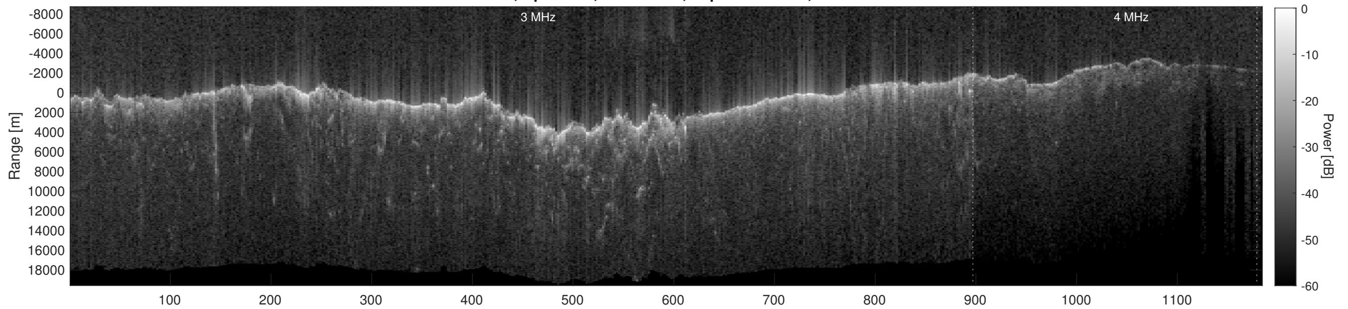
Orbit 8984, Depth-Corrected Cluttergram
