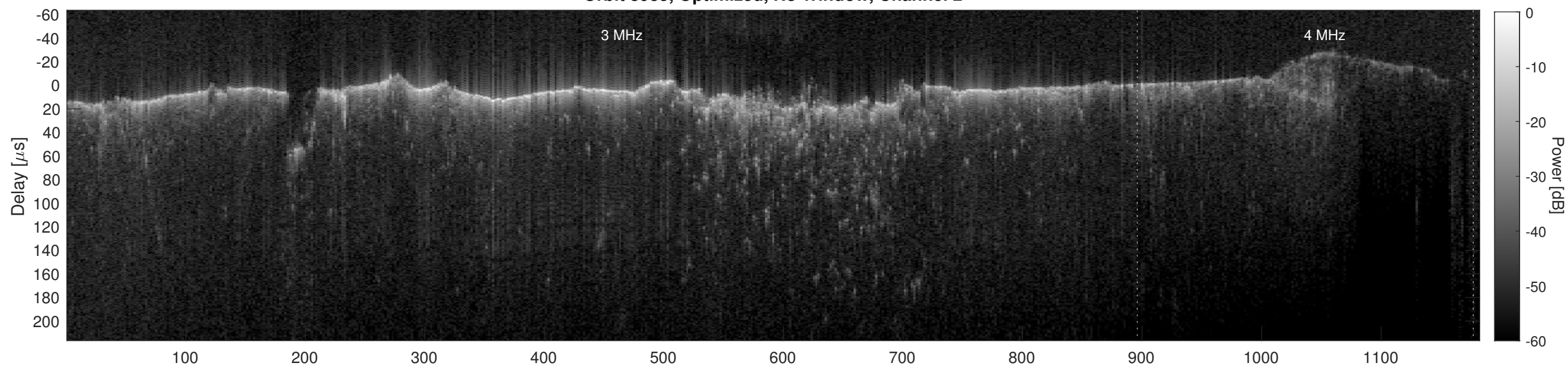
Orbit 8985, Cluttergram
