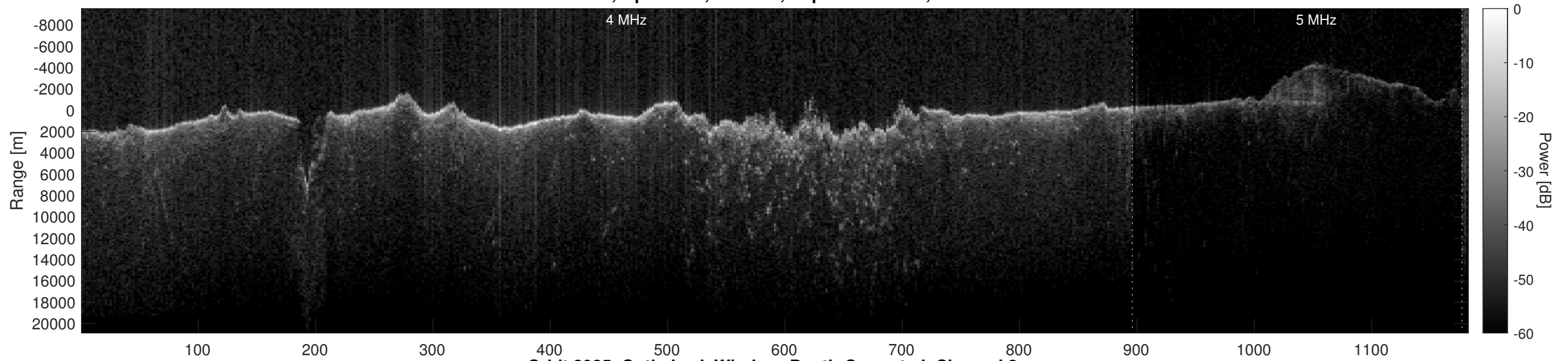
Orbit 8985, Optimized, Window, Depth-Corrected, Channel 2
