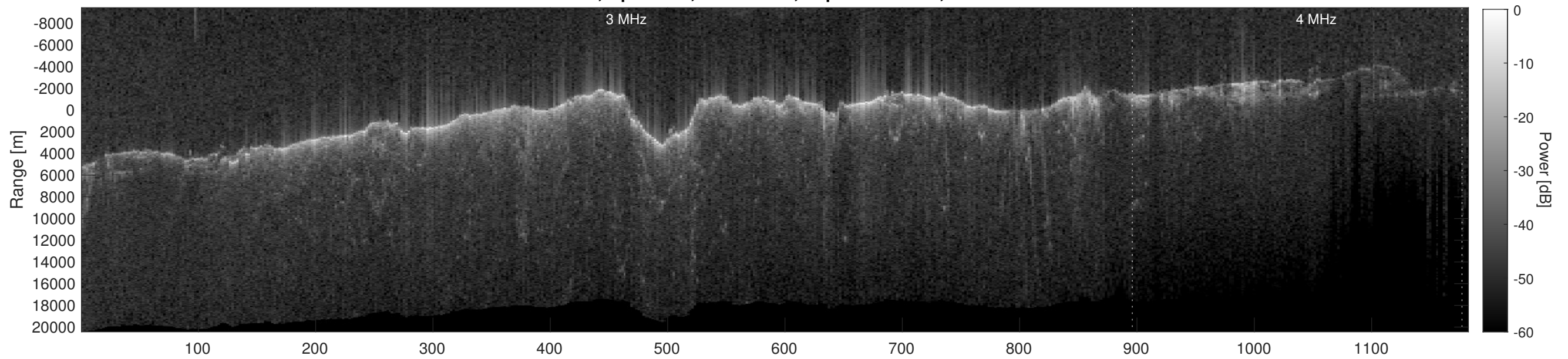
Orbit 8986, Depth-Corrected Cluttergram
