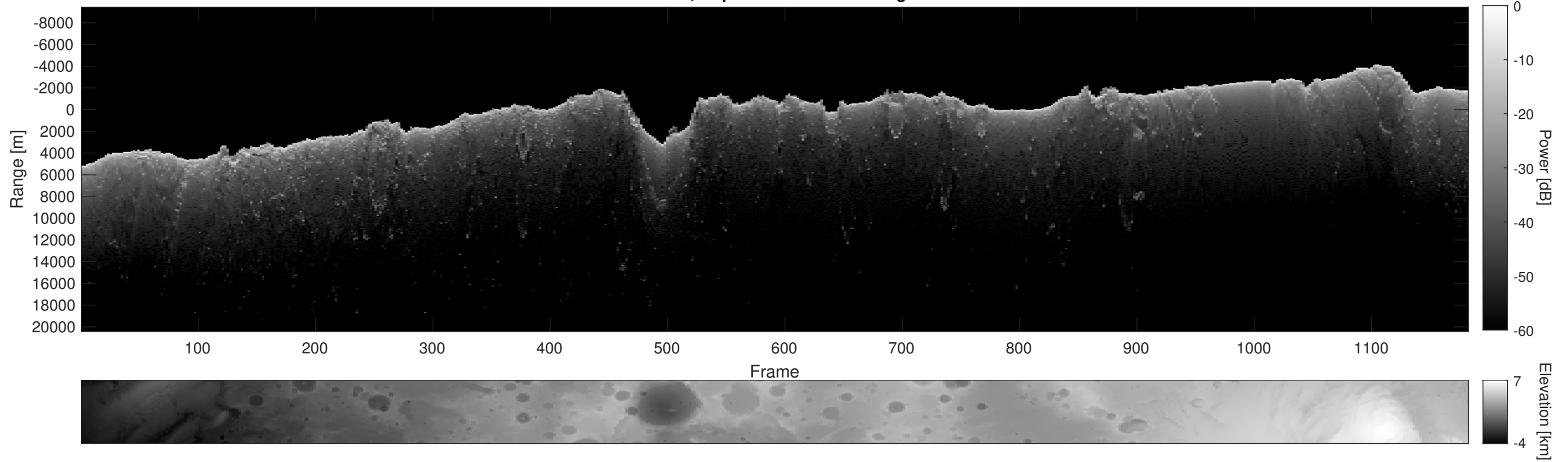
Orbit 8986, Depth-Corrected Cluttergram
