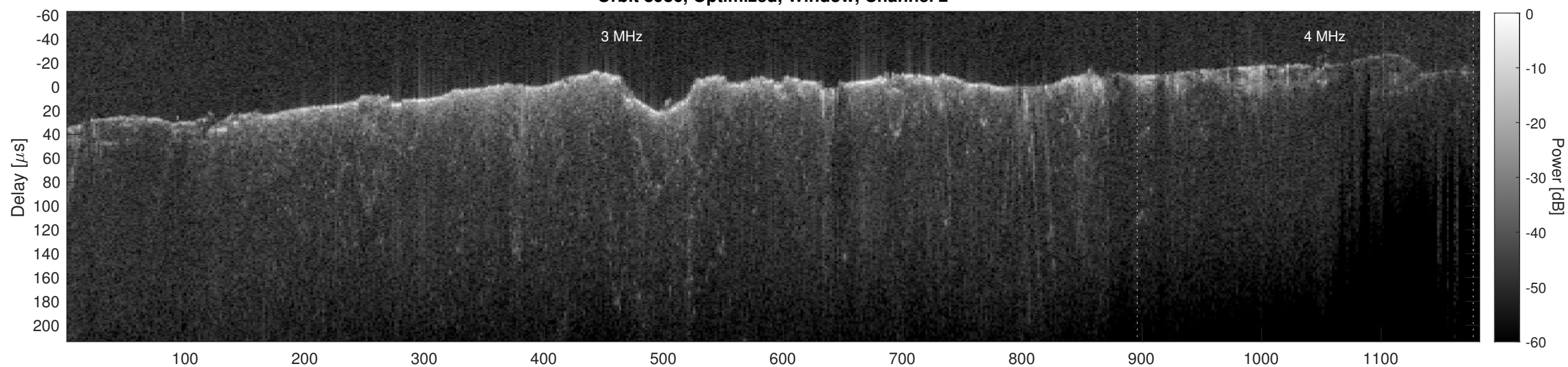
Orbit 8986, Cluttergram
