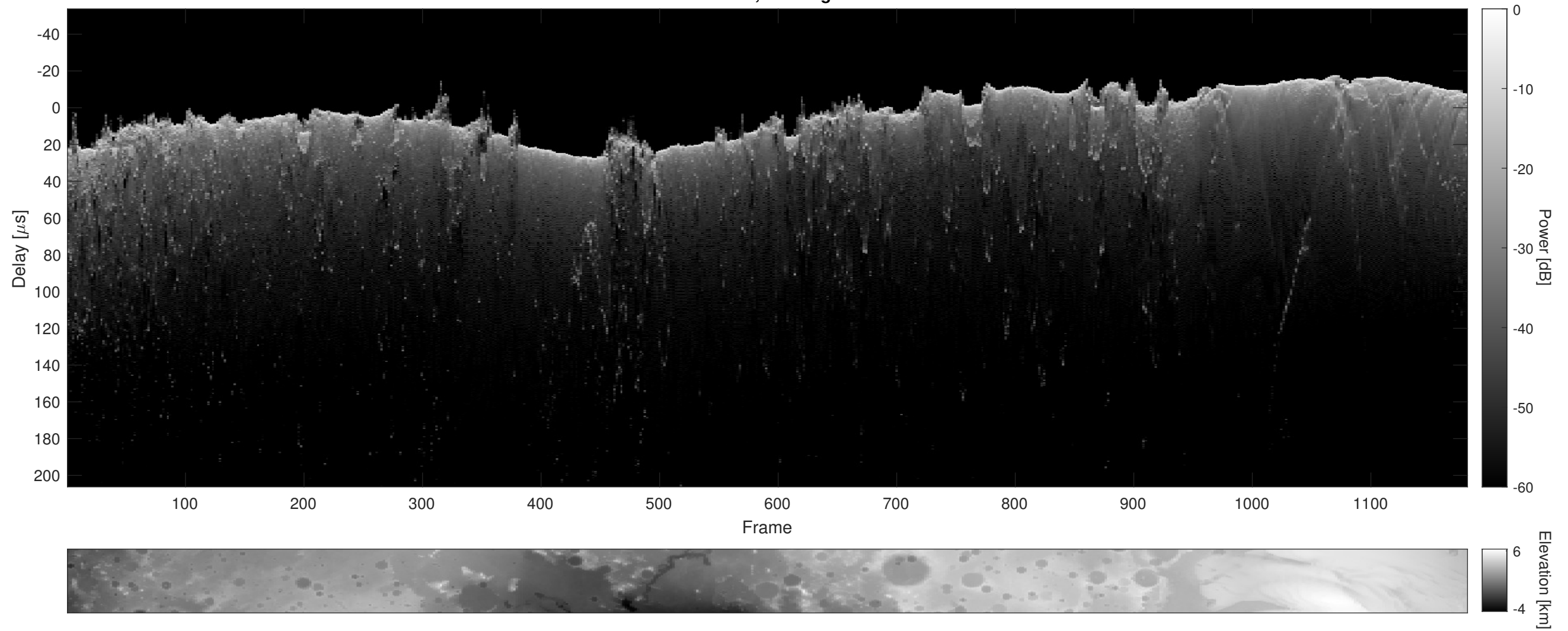
Orbit 8987, Cluttergram
