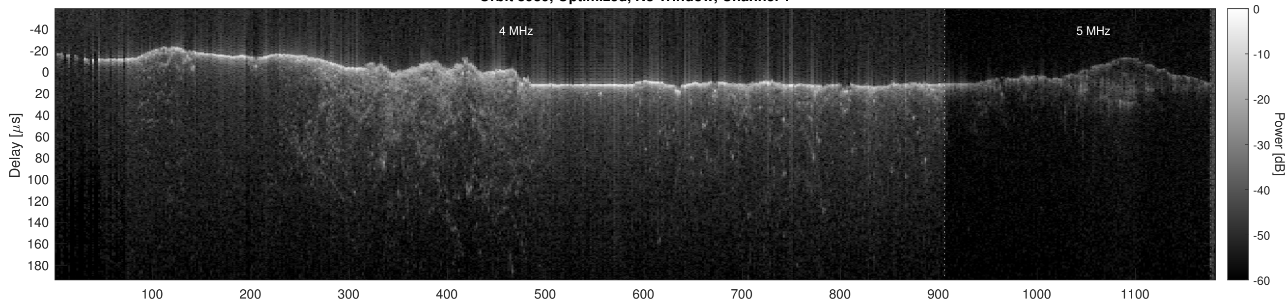
Orbit 8989, Optimized, No Window, Channel 2
