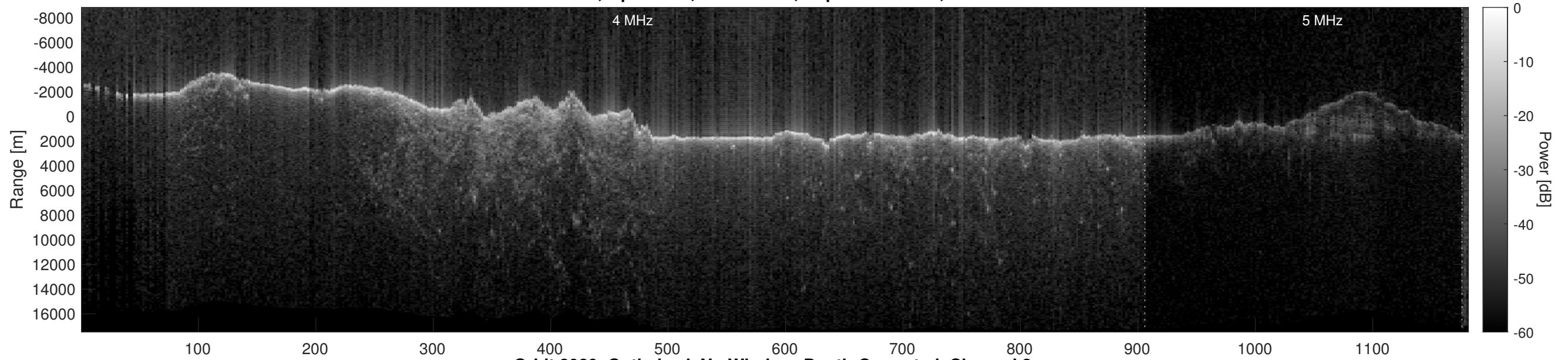
Orbit 8989, Optimized, No Window, Depth-Corrected, Channel 2
