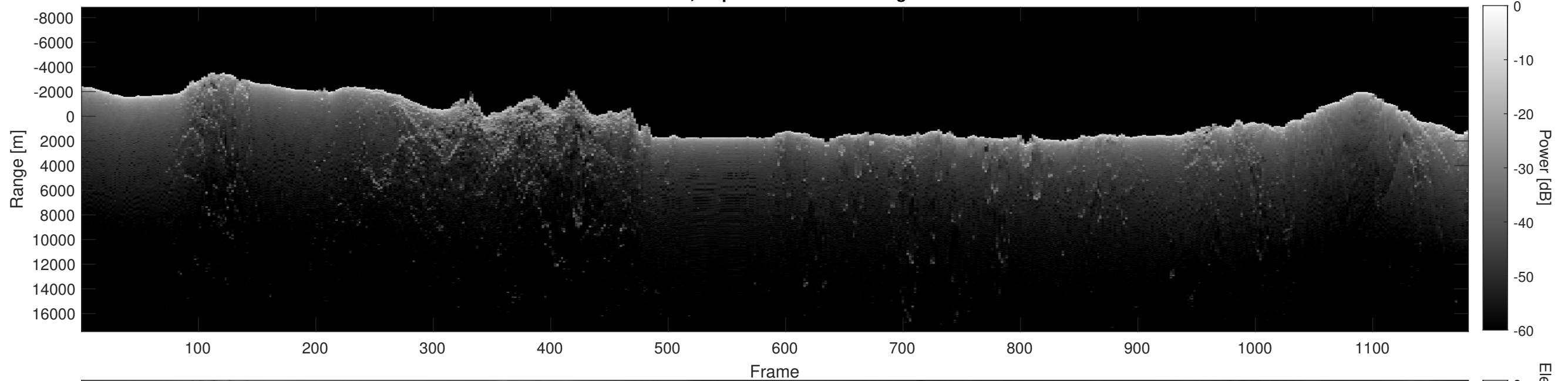
Orbit 8989, Depth-Corrected Cluttergram
