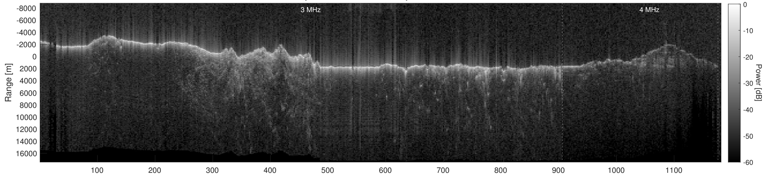
Orbit 8989, Depth-Corrected Cluttergram
