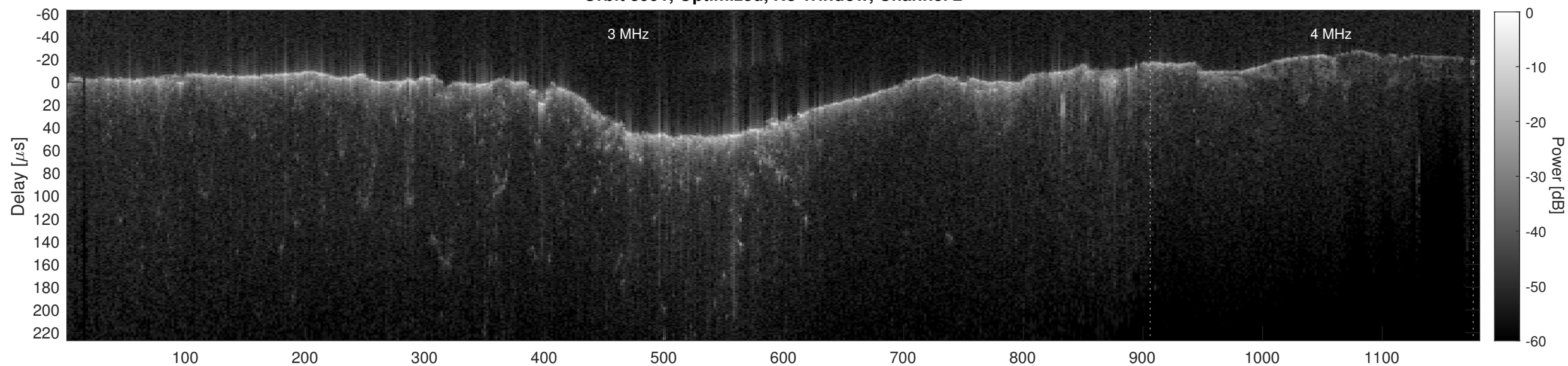
Orbit 8991, Cluttergram
