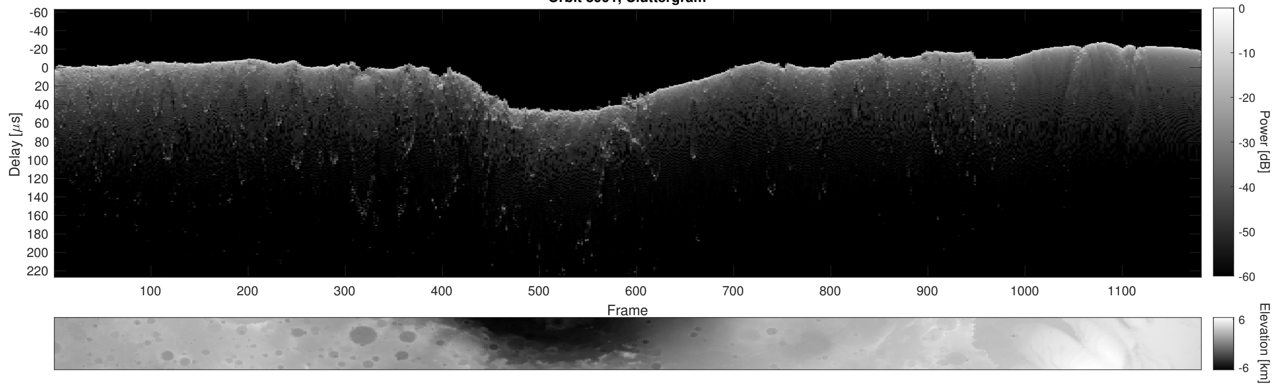
Orbit 8991, Cluttergram
