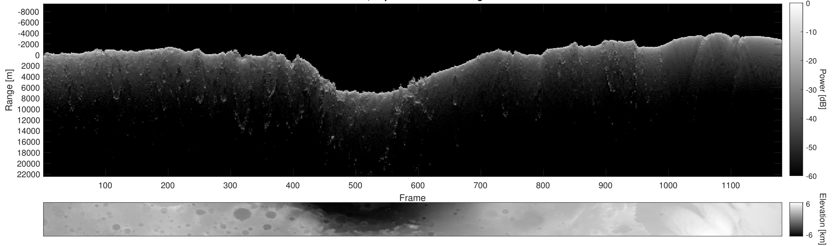
Orbit 8991, Depth-Corrected Cluttergram
