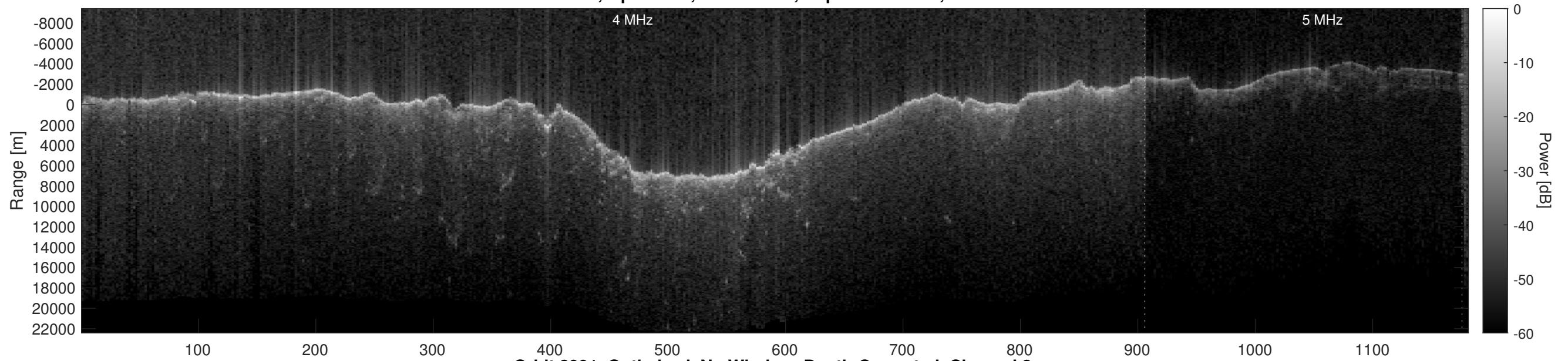
Orbit 8991, Optimized, No Window, Depth-Corrected, Channel 2
