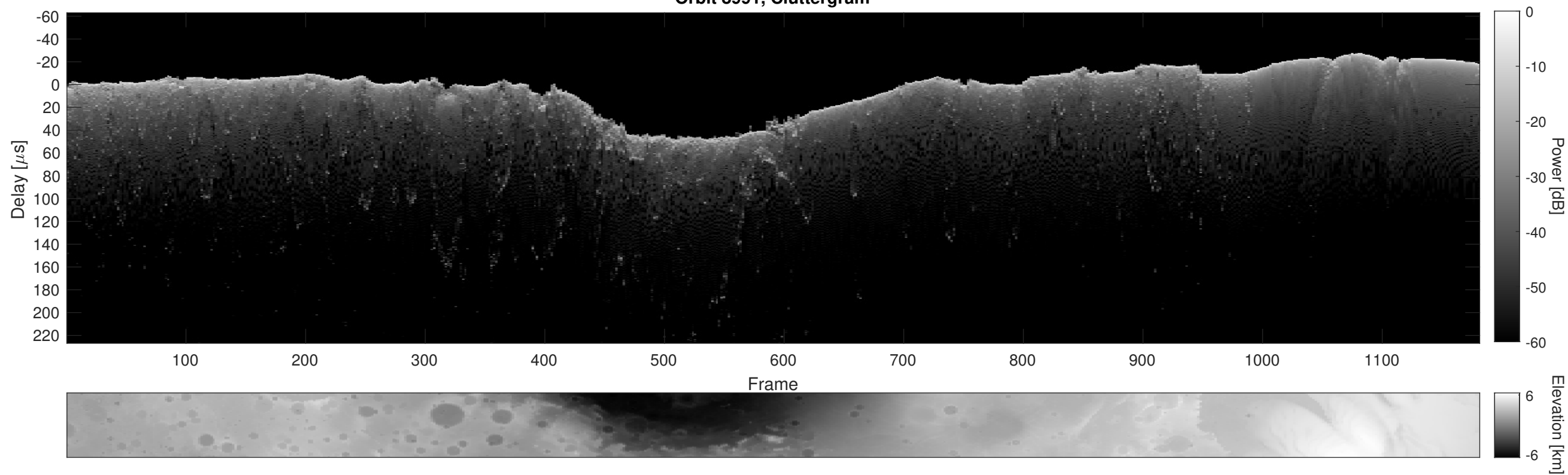
Orbit 8991, Cluttergram
