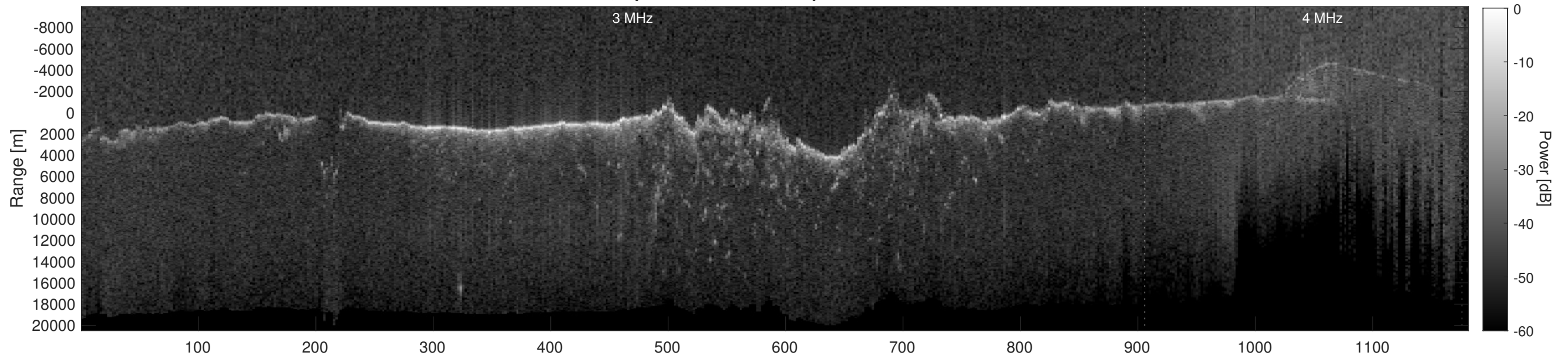
Orbit 8992, Depth-Corrected Cluttergram
