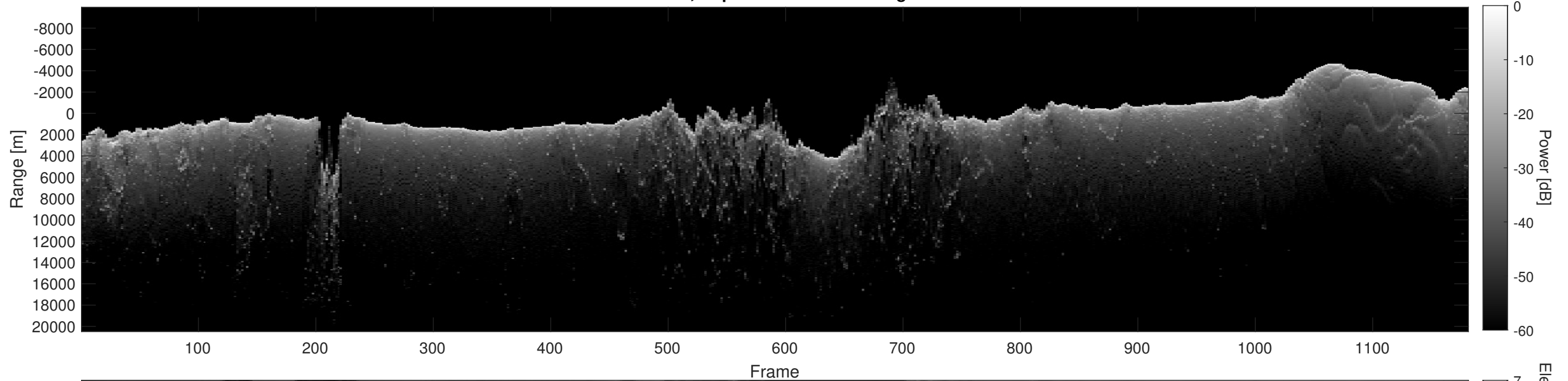
Orbit 8992, Depth-Corrected Cluttergram
