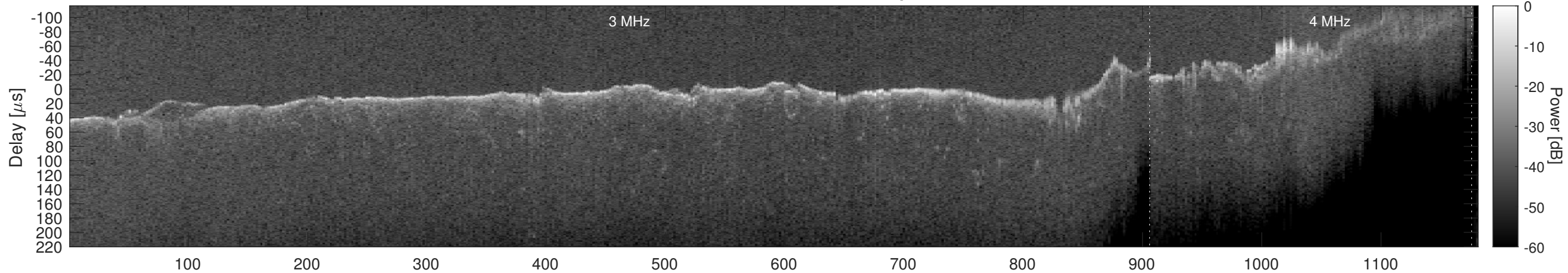
Orbit 8993, Window, Channel 2, Optimized
