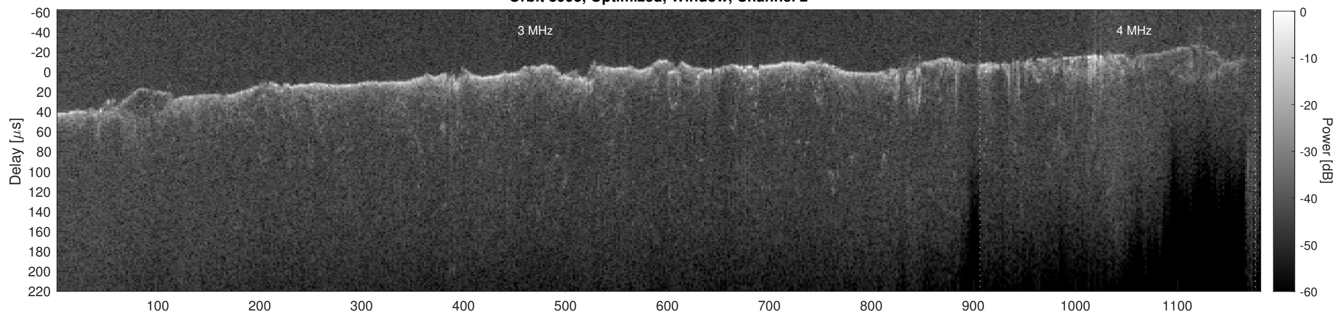
Orbit 8993, Cluttergram
