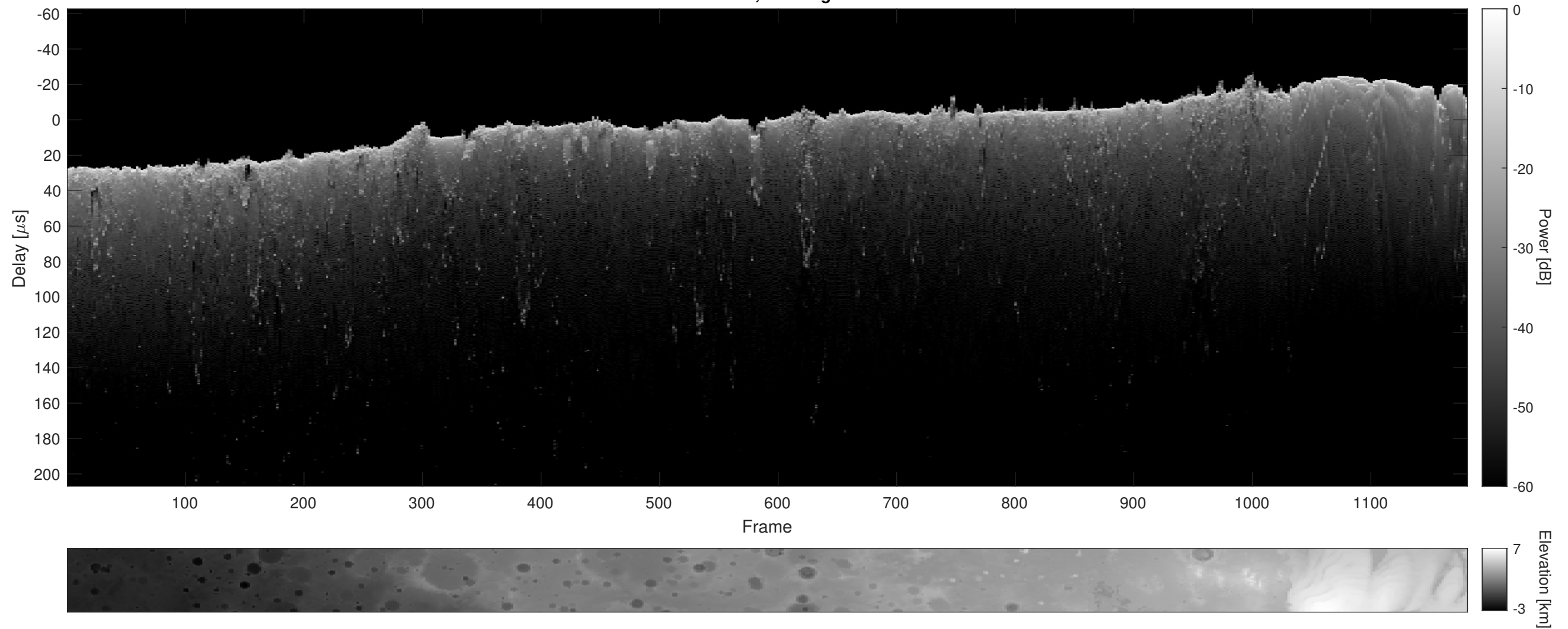
Orbit 8995, Cluttergram
