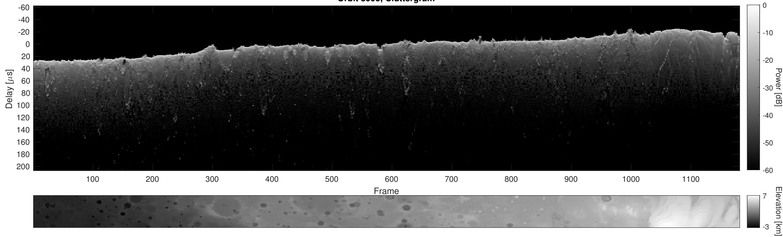
Orbit 8995, Cluttergram
