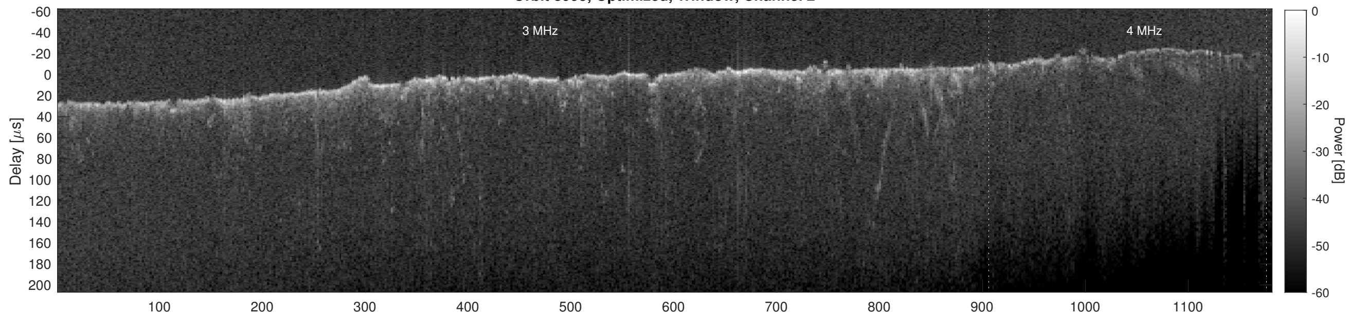
Orbit 8995, Cluttergram
