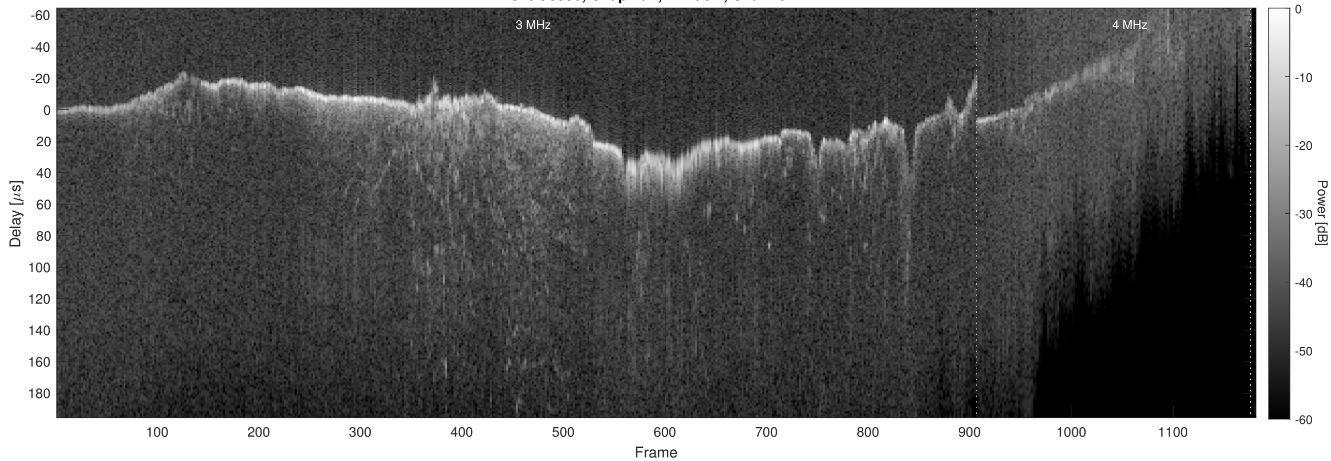
Orbit 8996, Chapman, Window, Channel 2
