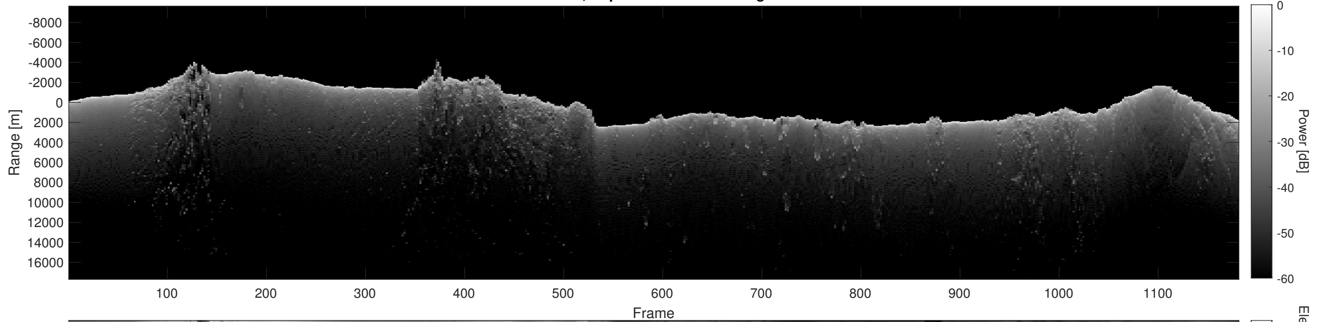
Orbit 8996, Depth-Corrected Cluttergram
