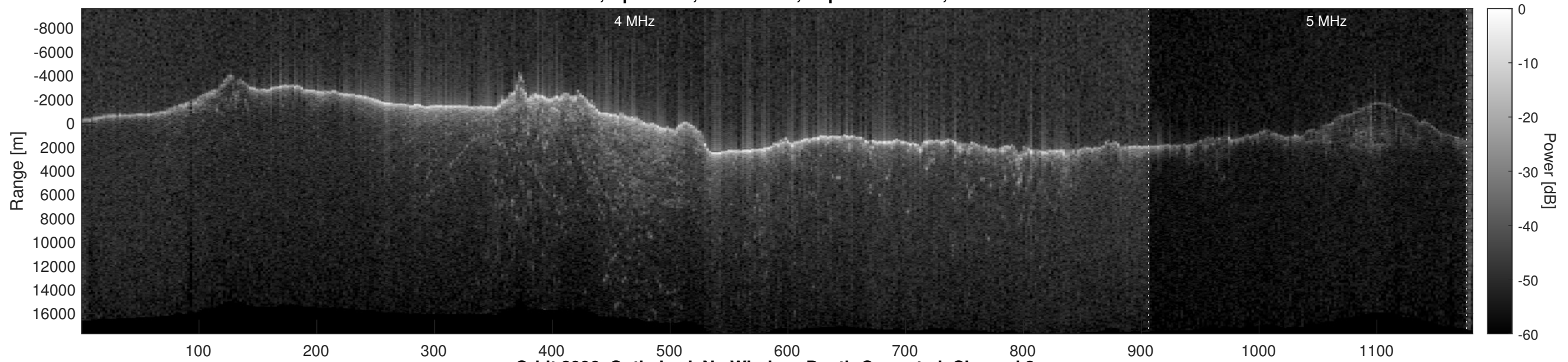
Orbit 8996, Optimized, No Window, Depth-Corrected, Channel 2
