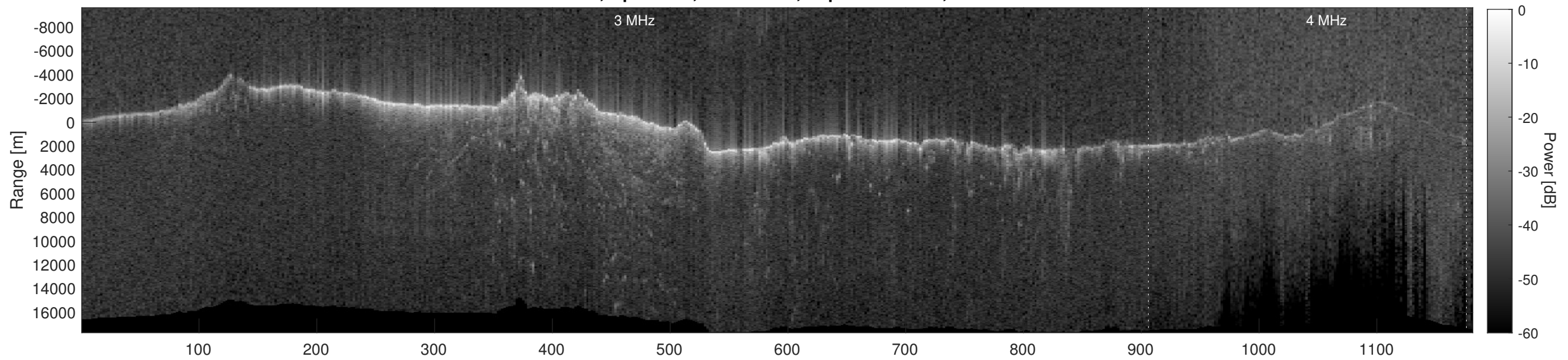
Orbit 8996, Depth-Corrected Cluttergram
