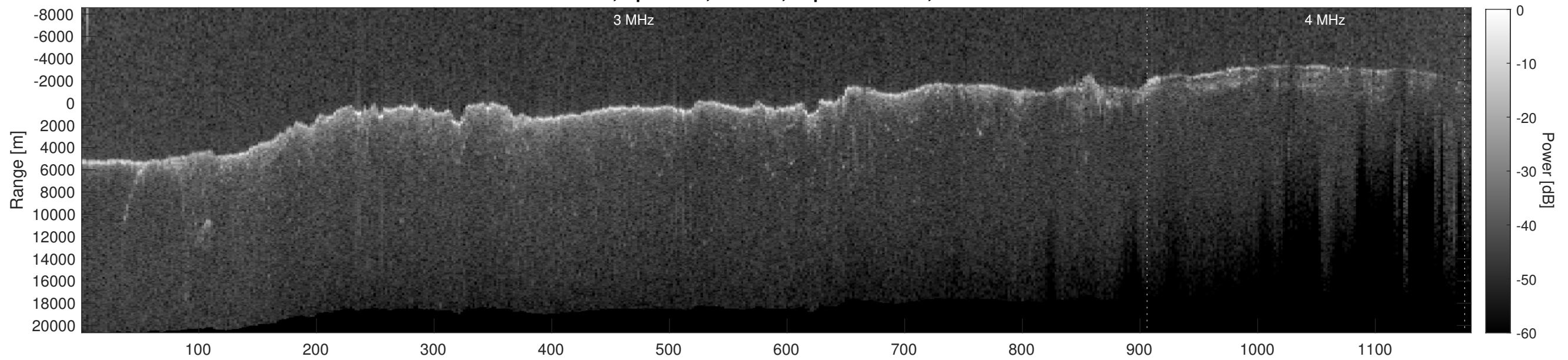
Orbit 8997, Depth-Corrected Cluttergram
