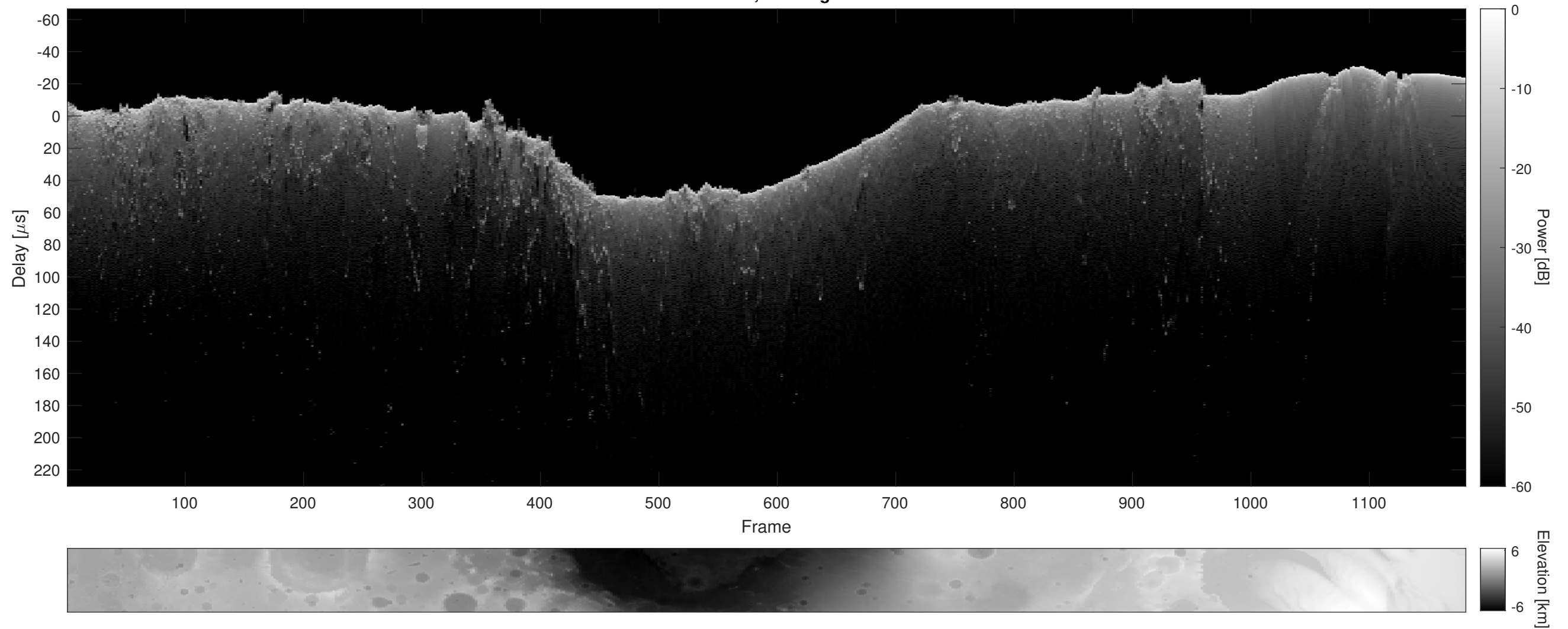
Orbit 8998, Cluttergram
