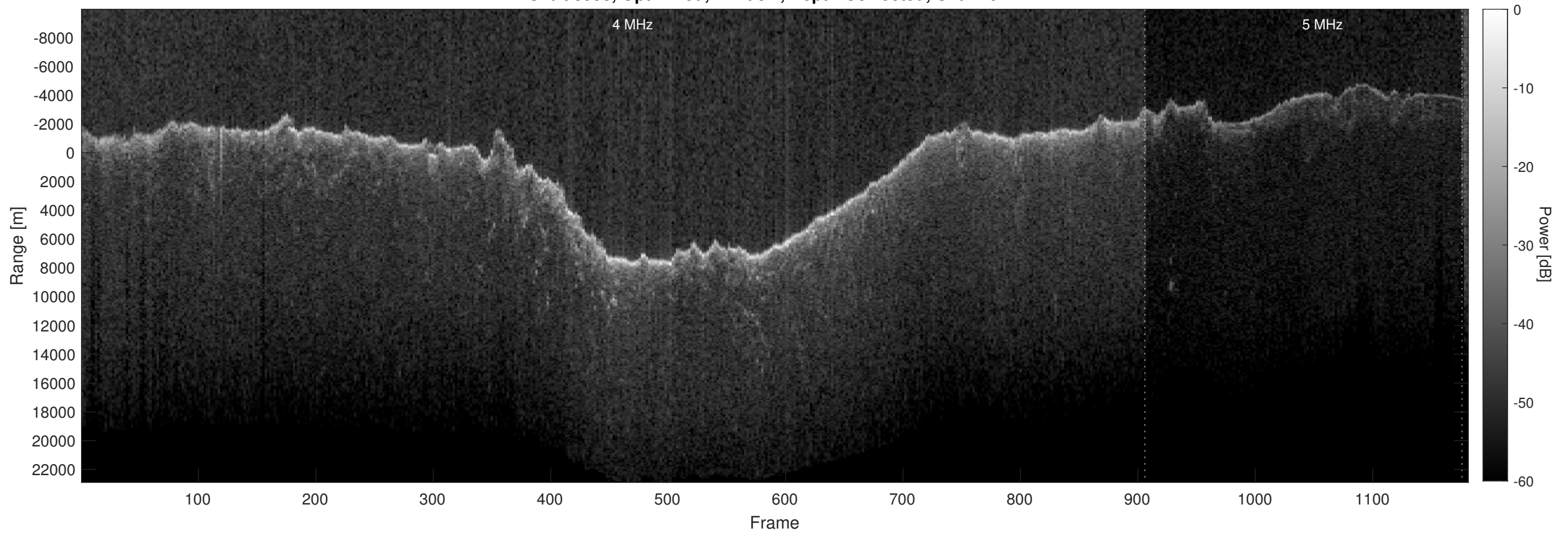
Orbit 8998, Optimized, Window, Depth-Corrected, Channel 2
