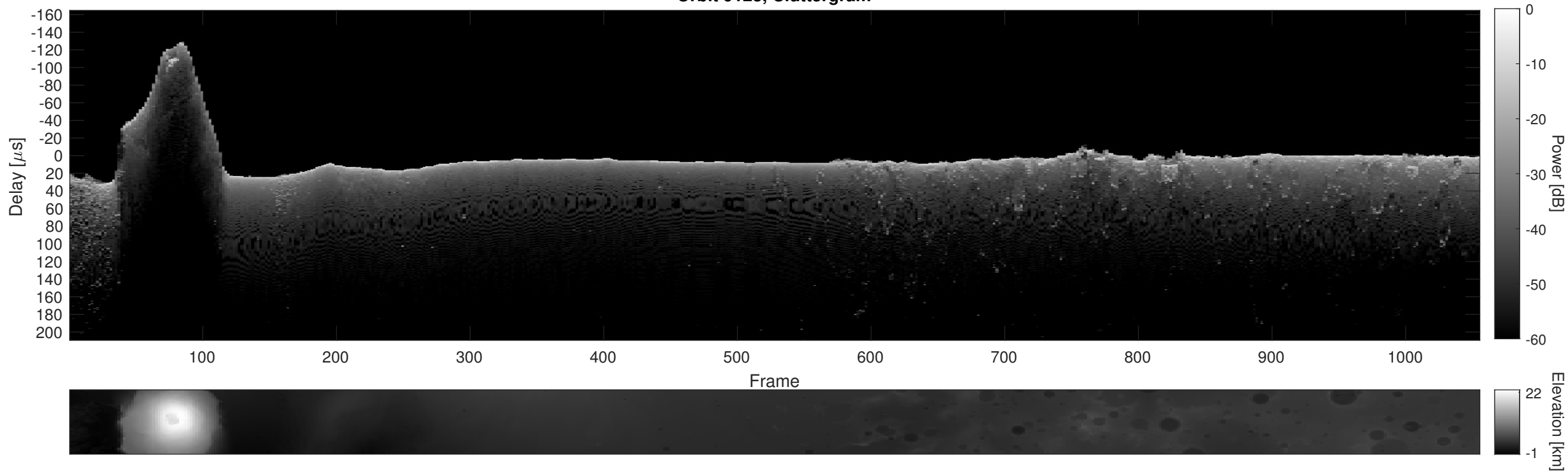
Orbit 9123, Cluttergram
