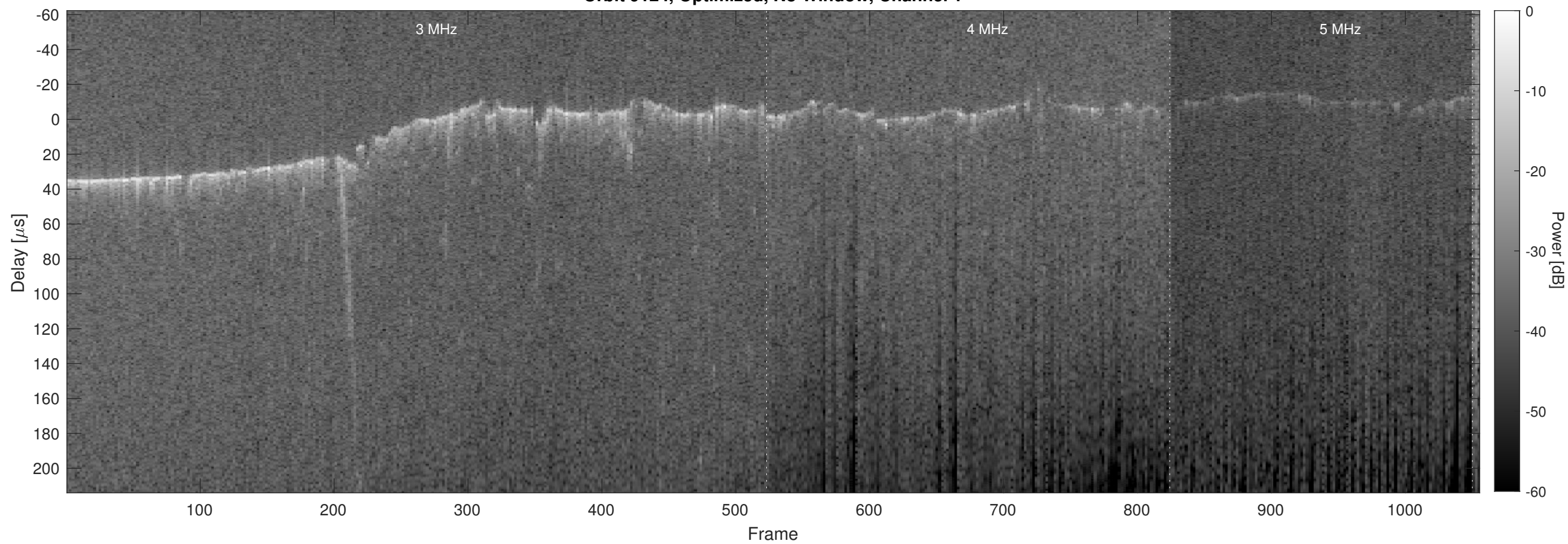
Orbit 9124, Optimized, No Window, Channel 2
