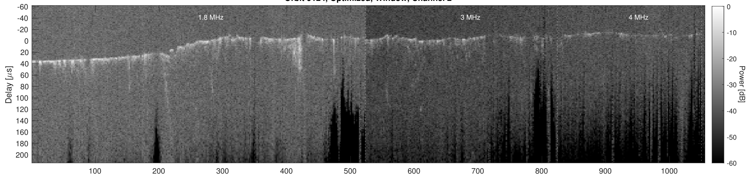
Orbit 9124, Cluttergram
