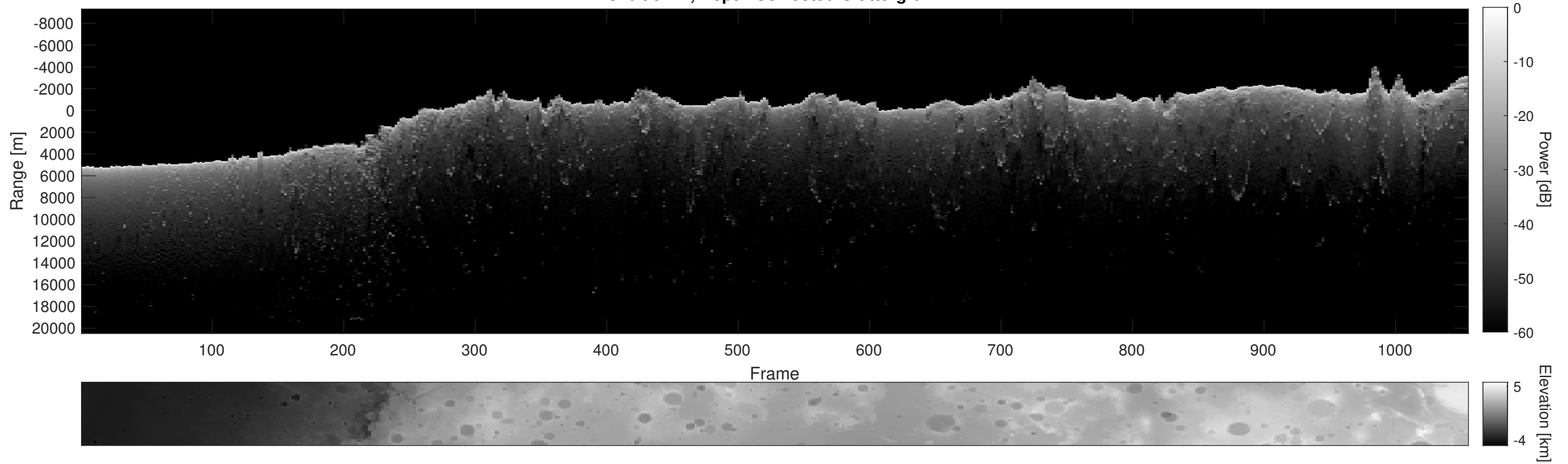
Orbit 9124, Depth-Corrected Cluttergram
