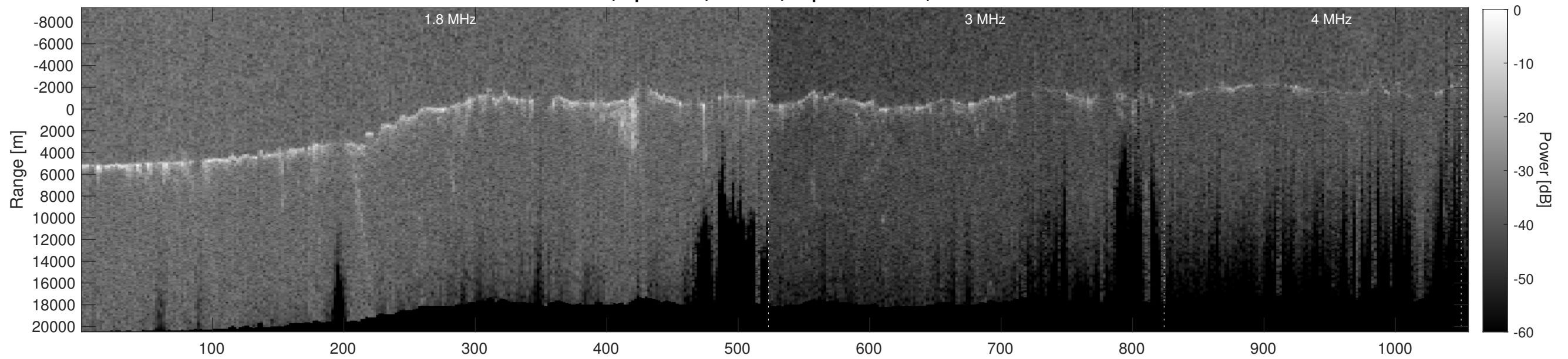
Orbit 9124, Depth-Corrected Cluttergram
