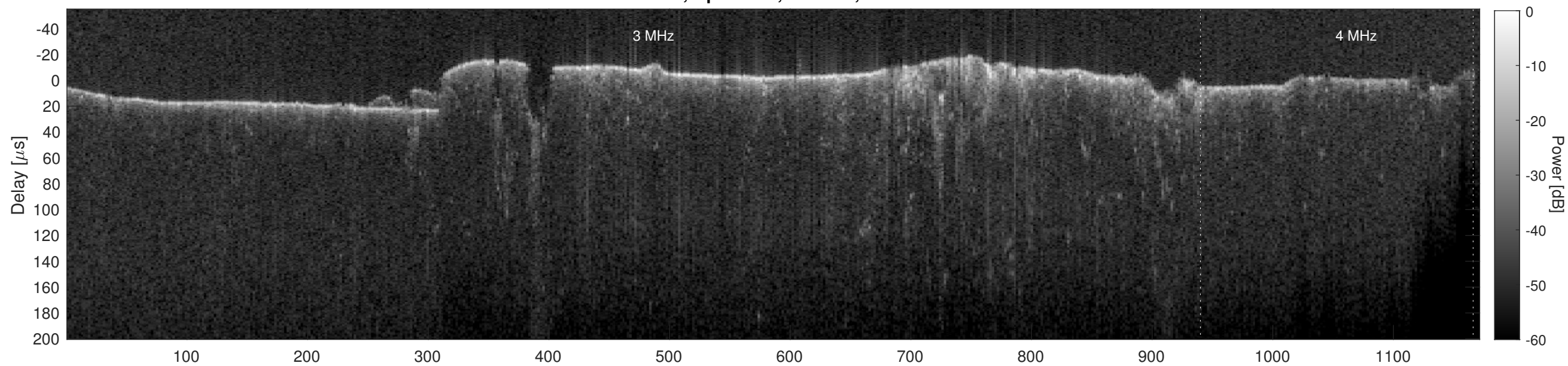
Orbit 9126, Cluttergram
