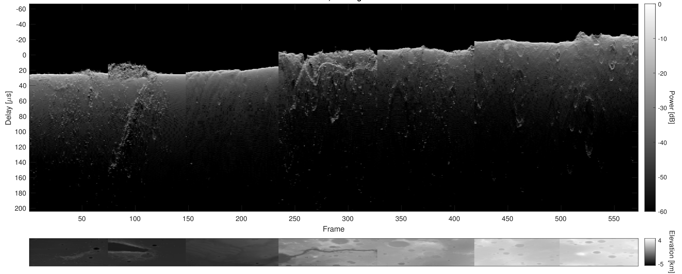
Orbit 9127, Cluttergram
