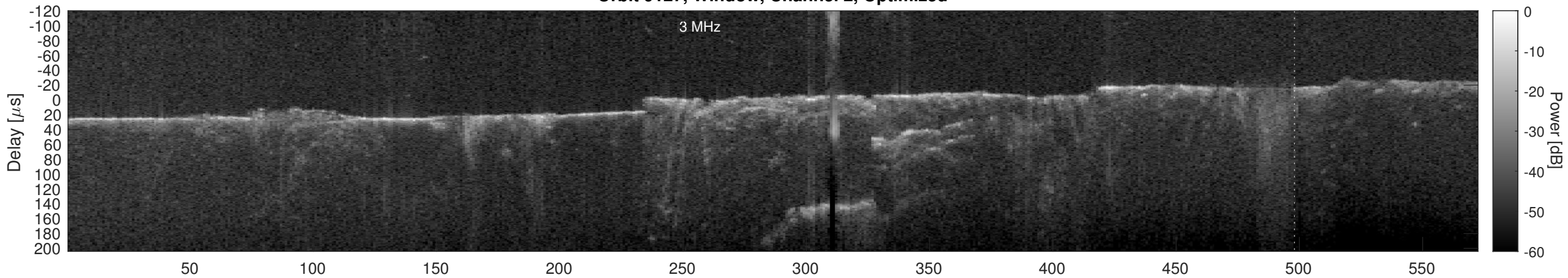
Orbit 9127, Cluttergram
