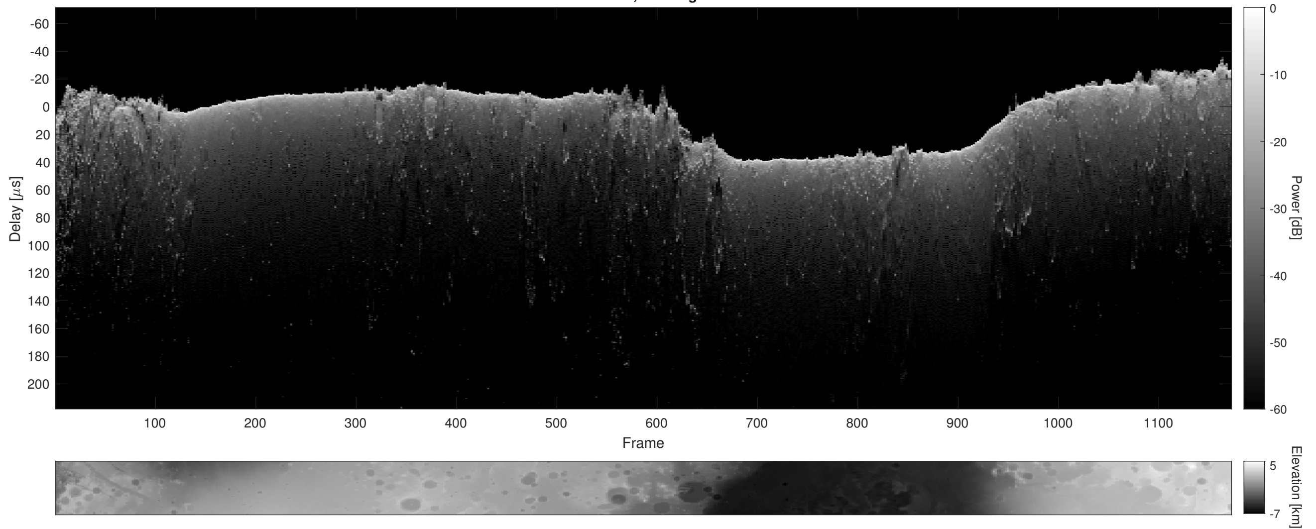
Orbit 9128, Cluttergram
