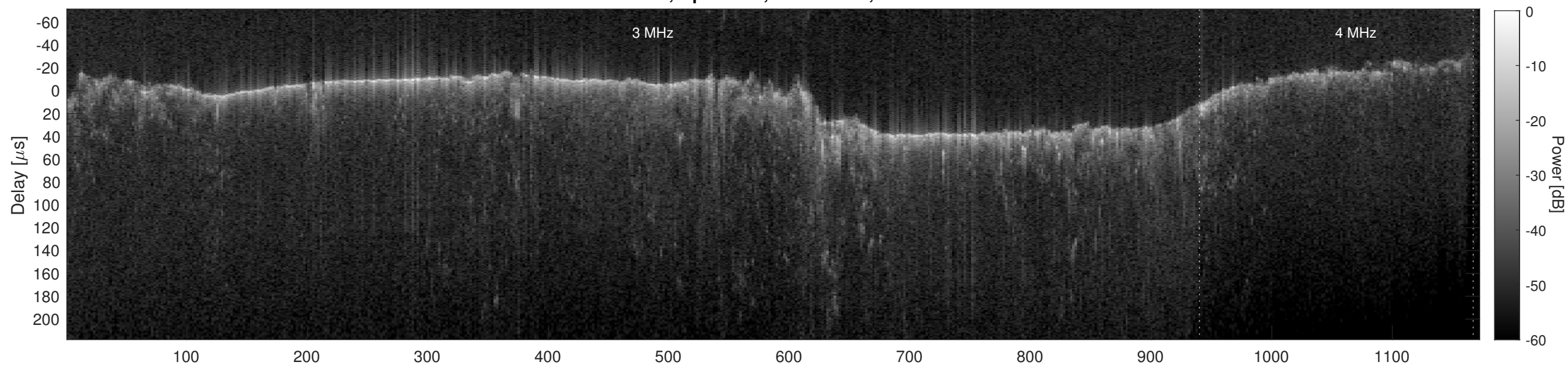
Orbit 9128, Cluttergram
