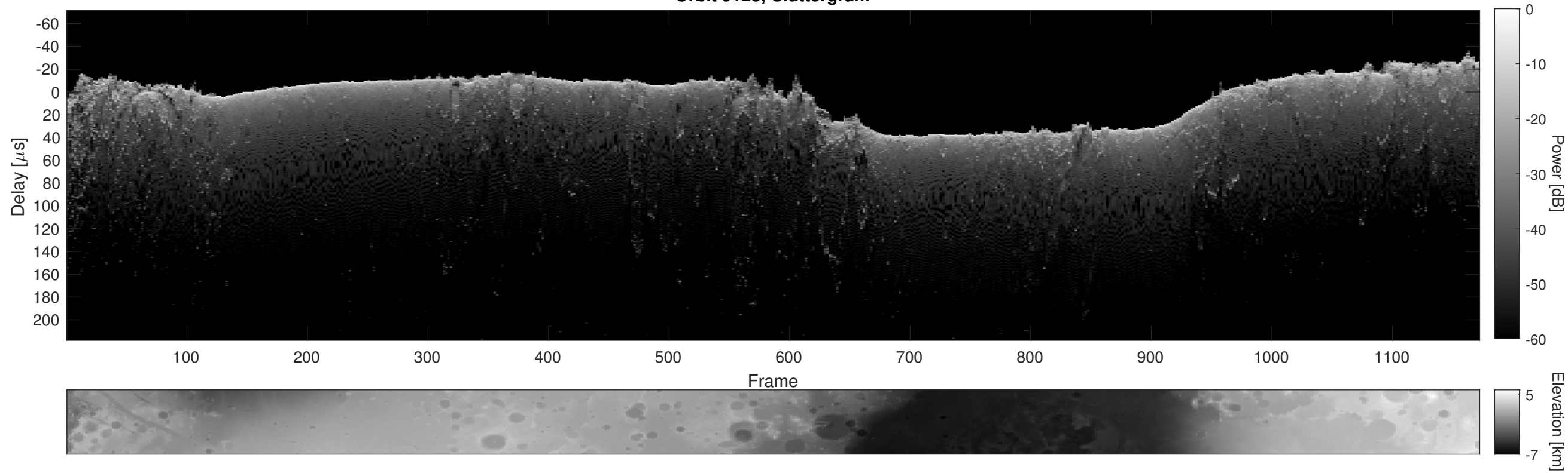
Orbit 9128, Cluttergram
