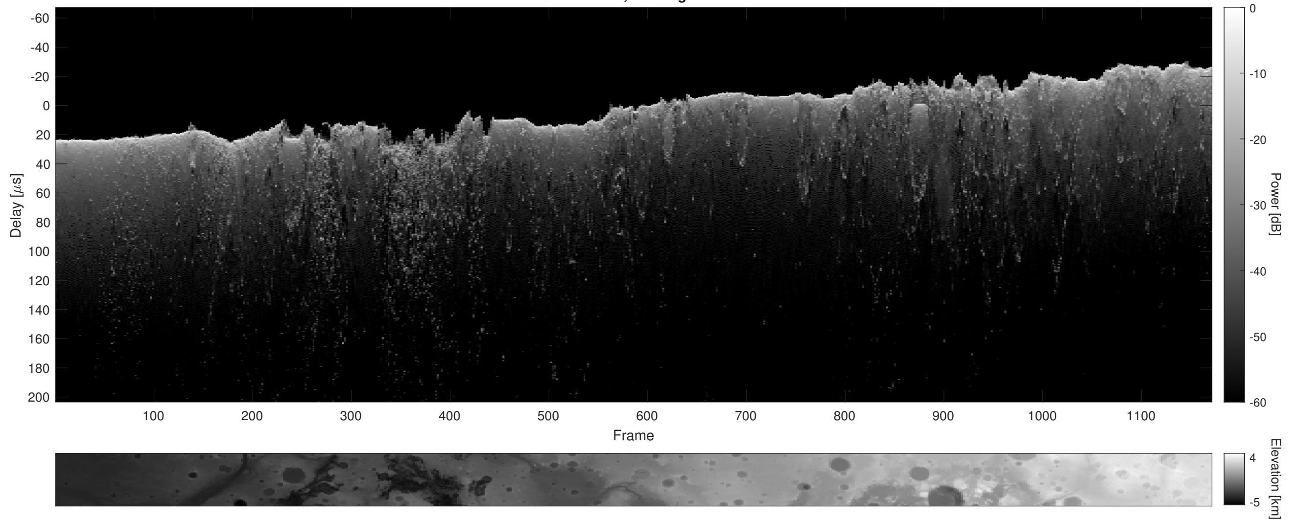
Orbit 9129, Cluttergram
