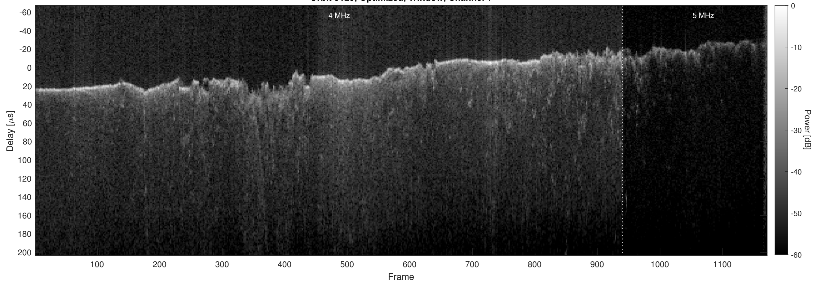
Orbit 9129, Optimized, Window, Channel 2
