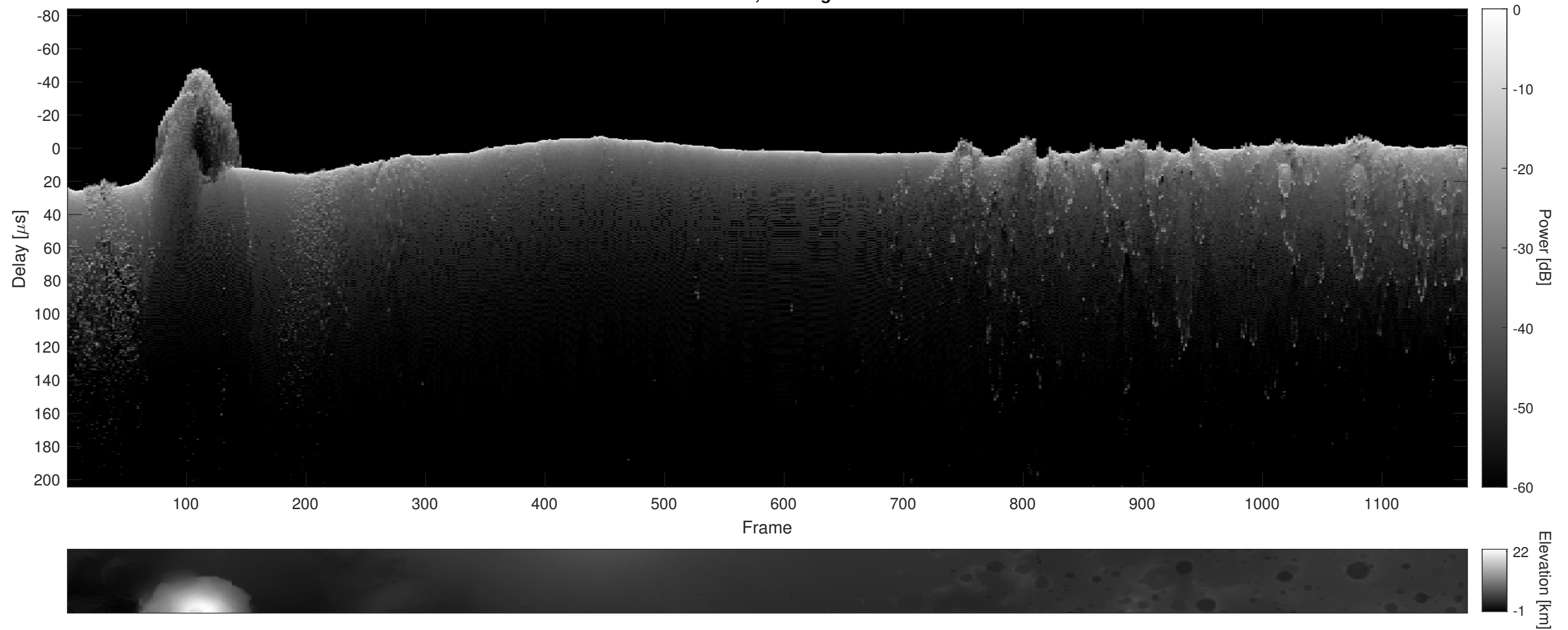
Orbit 9130, Cluttergram
