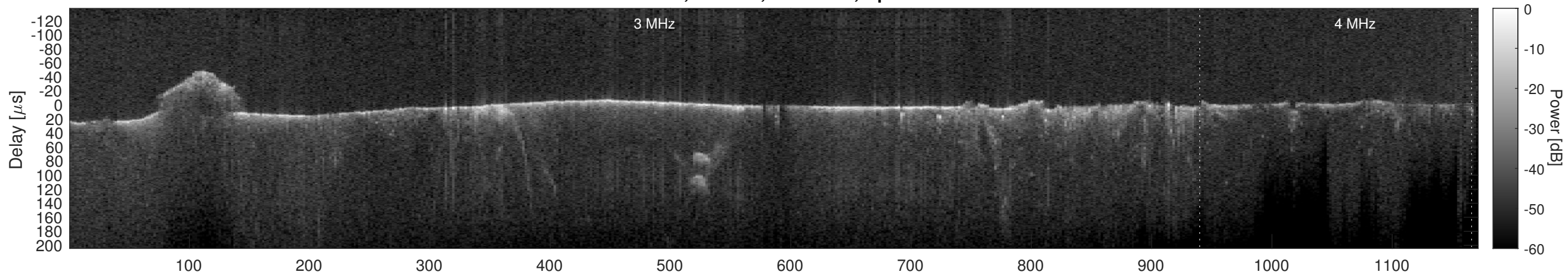
Orbit 9130, Cluttergram
