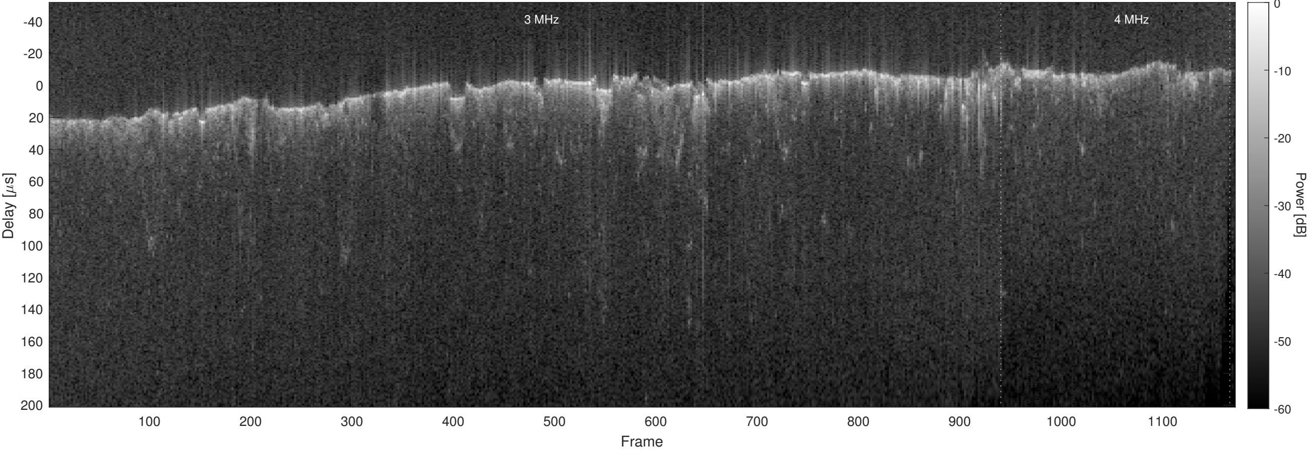
Orbit 9132, Optimized, No Window, Channel 2
