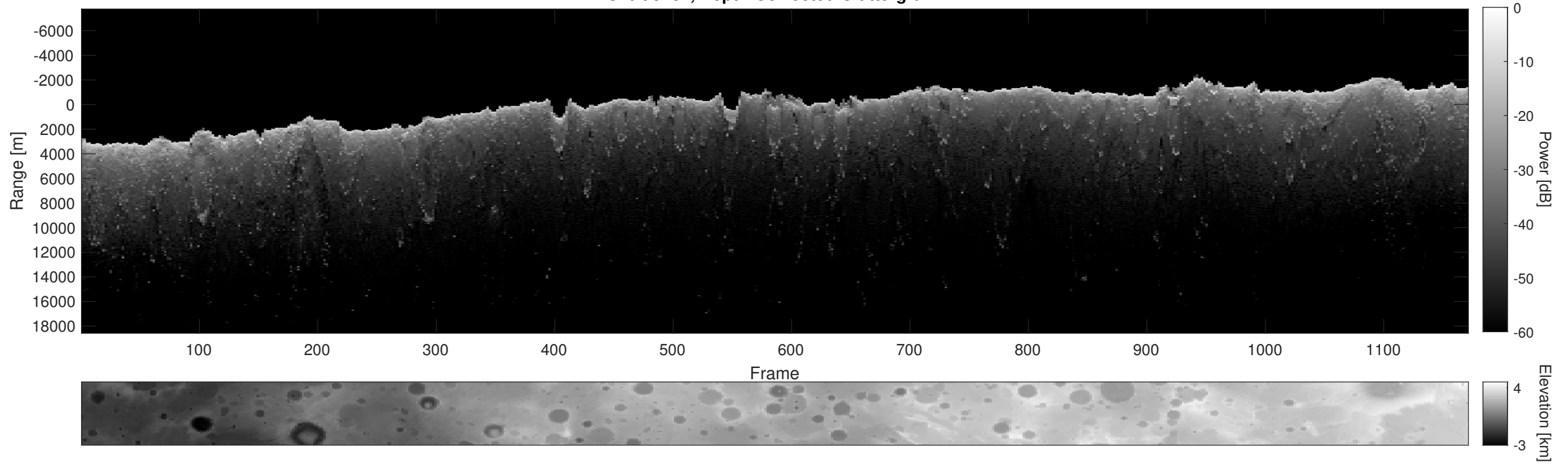
Orbit 9132, Depth-Corrected Cluttergram
