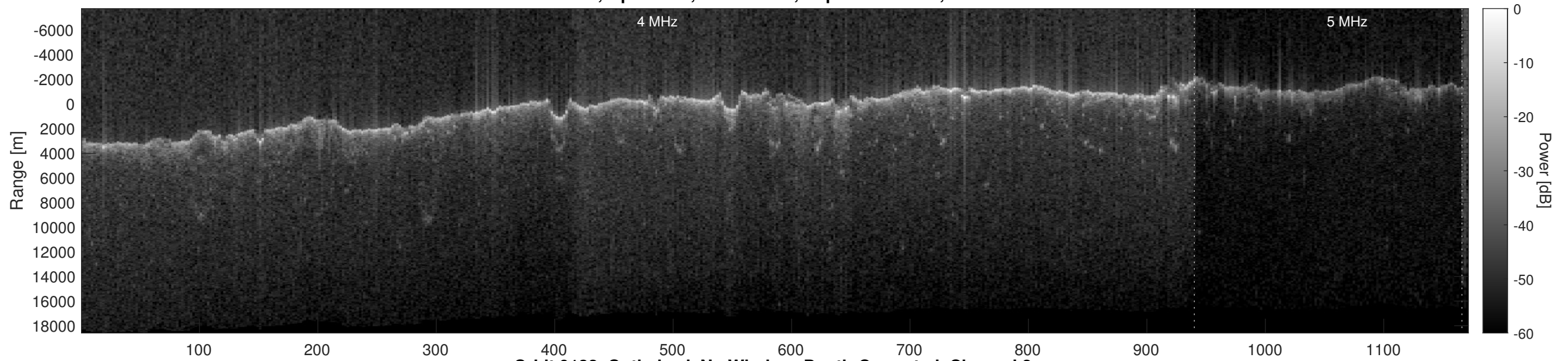
Orbit 9132, Optimized, No Window, Depth-Corrected, Channel 2
