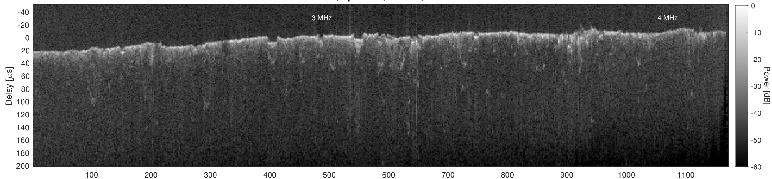
Orbit 9132, Cluttergram
