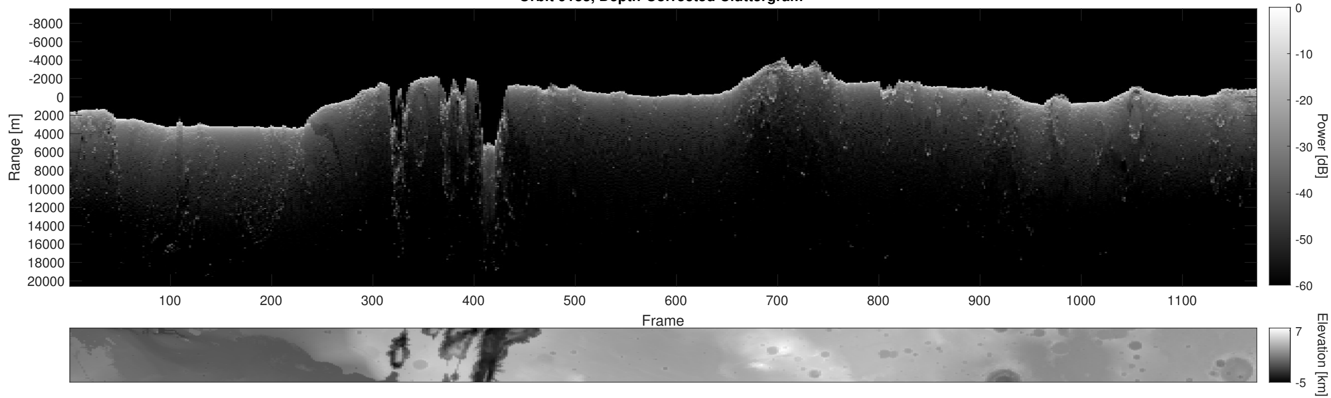
Orbit 9133, Depth-Corrected Cluttergram
